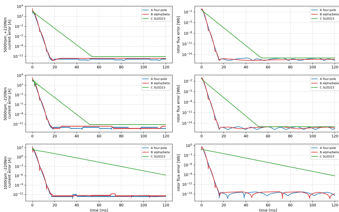
Nominal convergence comparison of three observer gain-design methods
