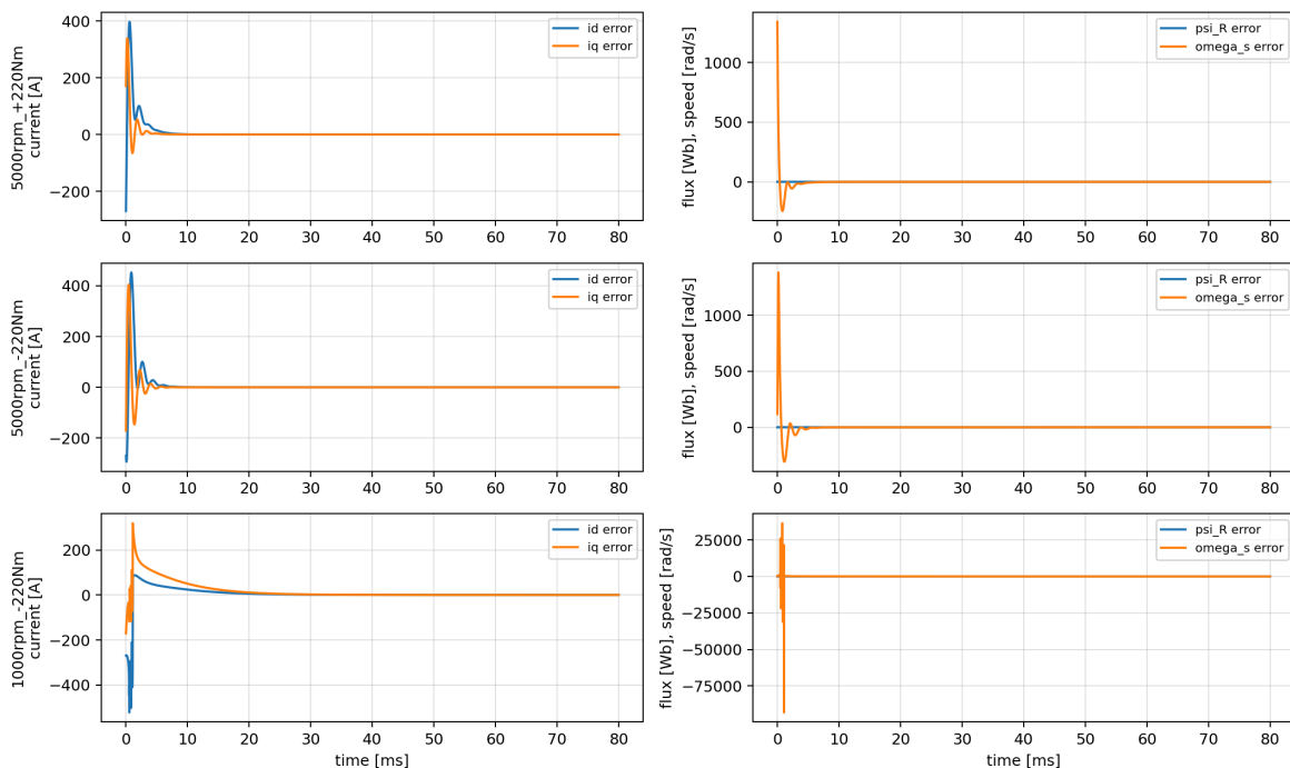
SLED 2023 Appendix A observer convergence
