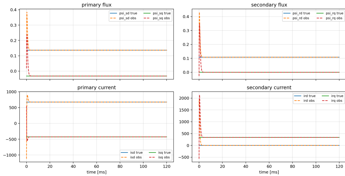
Nominal waveform convergence at 1000 r/min, -220 Nm
