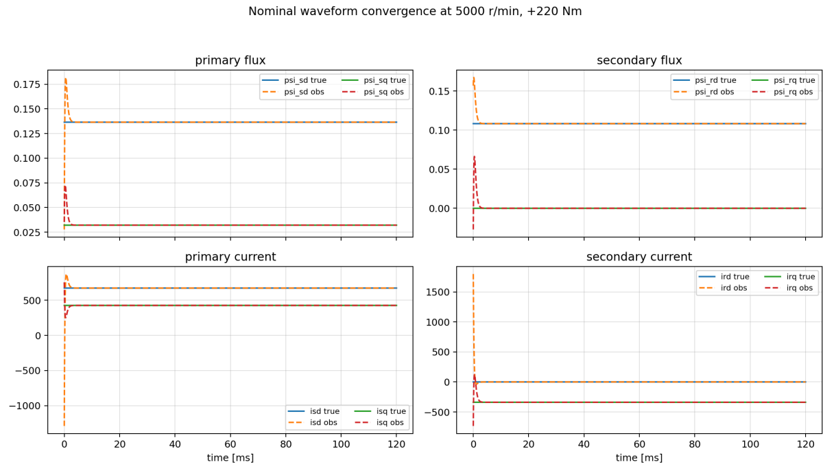
5000 r/min motoring nominal waveform
