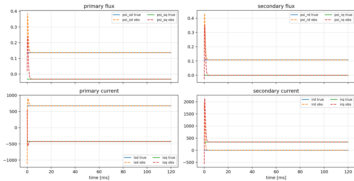
1000 r/min regeneration nominal waveform
