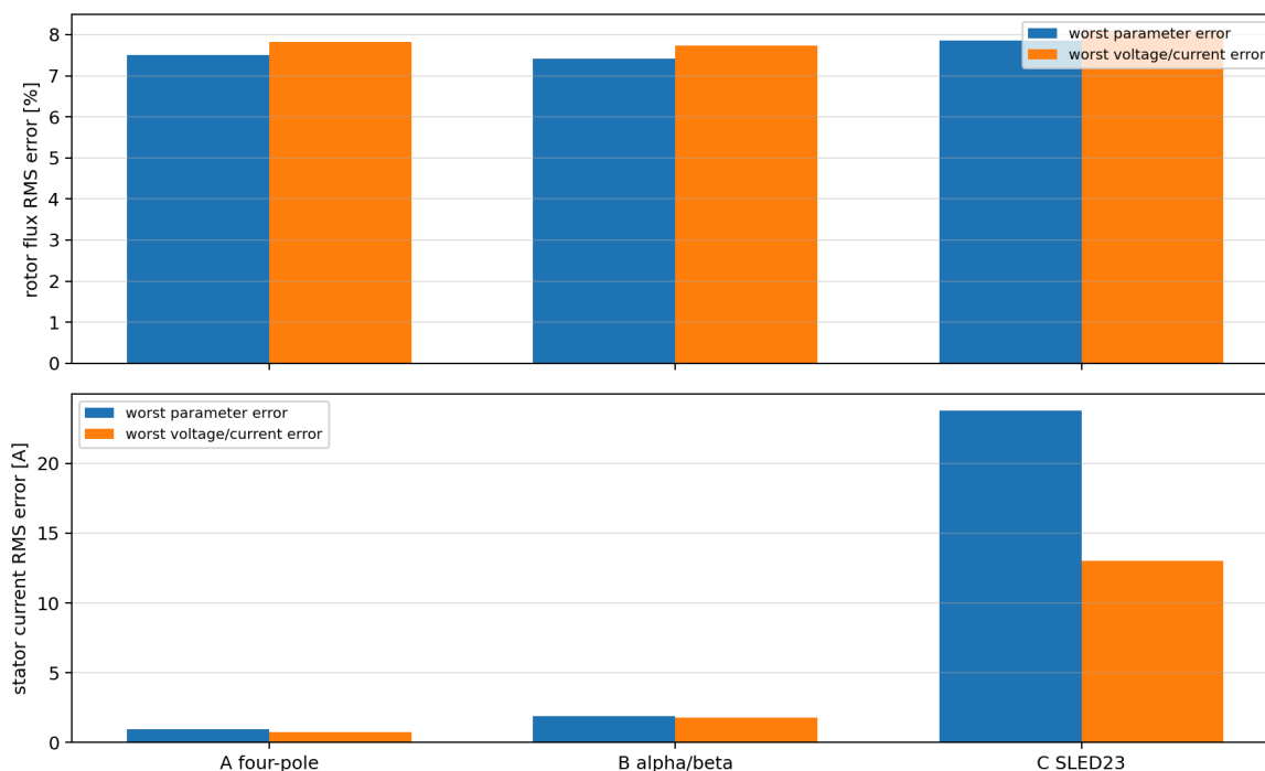
Worst error comparison at 5000 r/min, -220 Nm
