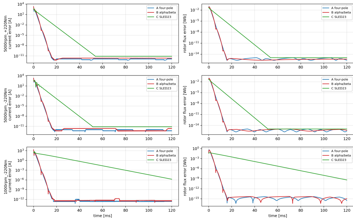
Nominal convergence comparison of three observer gain-design methods
