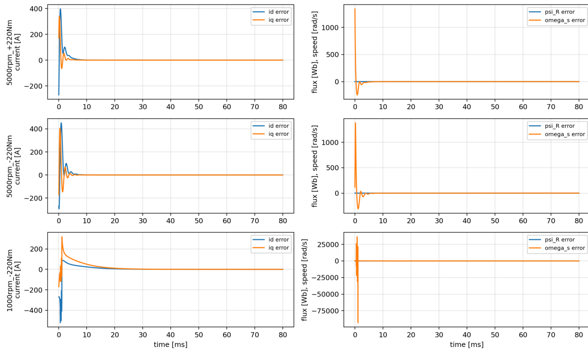
sled23 appendix observer convergence
