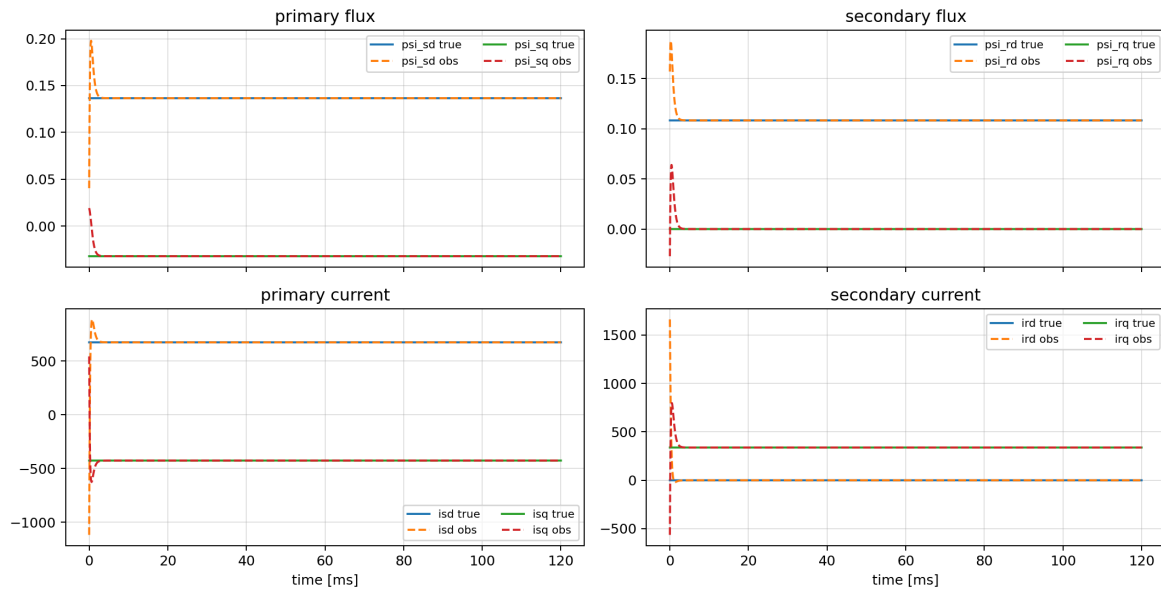
5000 r/min regeneration nominal waveform
