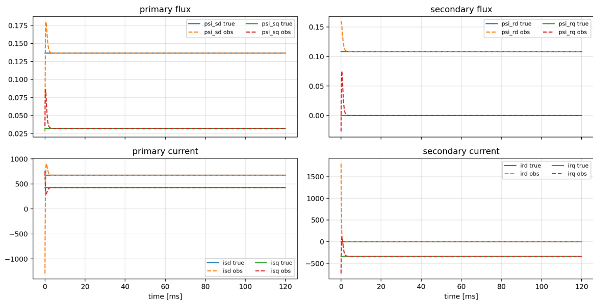
Nominal waveform convergence at 5000 r/min, +220 Nm
