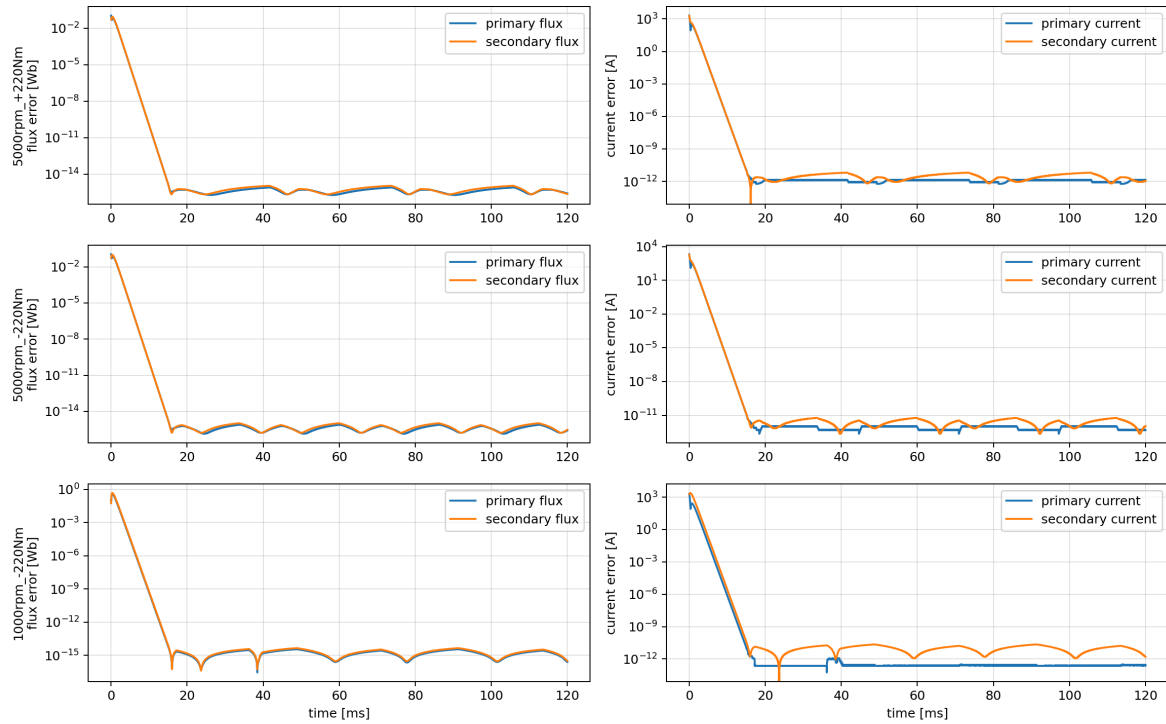
Nominal observer convergence from initial flux error
