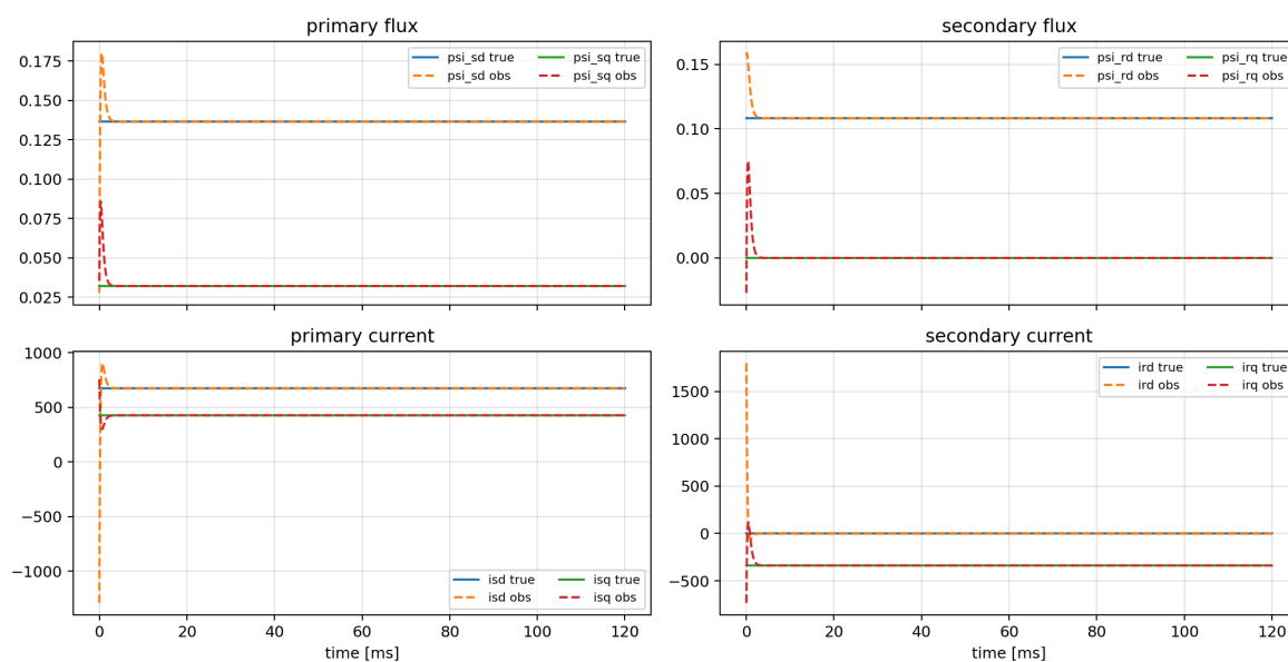
5000 r/min motoring nominal waveform
