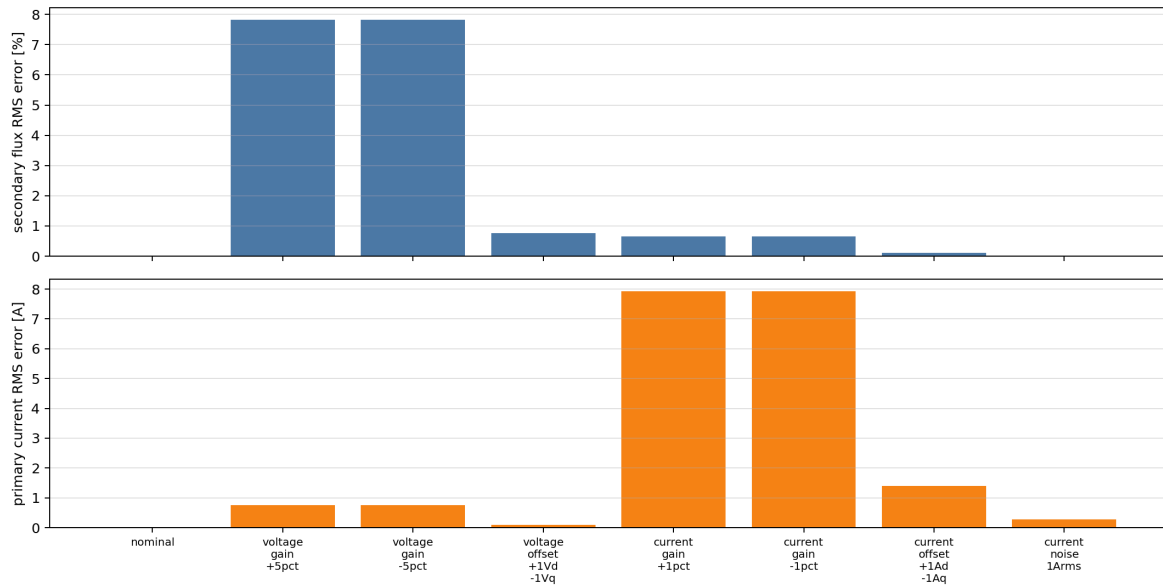
Voltage/current measurement error sensitivity at 5000 r/min, -220 Nm
