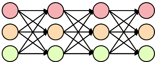
Searchable Backbone
