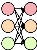
Searchable Head
