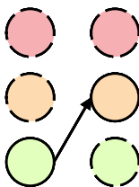
Searched Head
