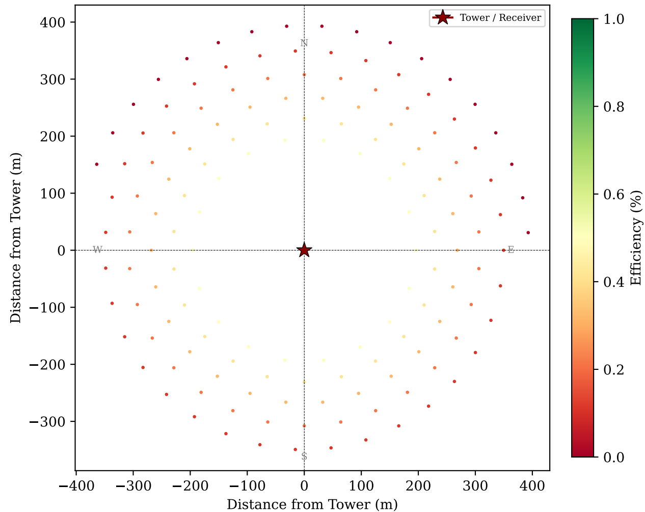
ML-GA Eff-opt Radial TH=260.9m, LH=18.95m, N=149
