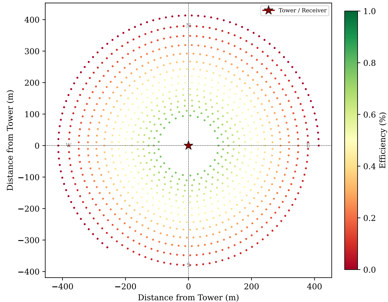
ML-GA LCOE-opt Radial TH=126.9m, LH=8.23m, N=981
