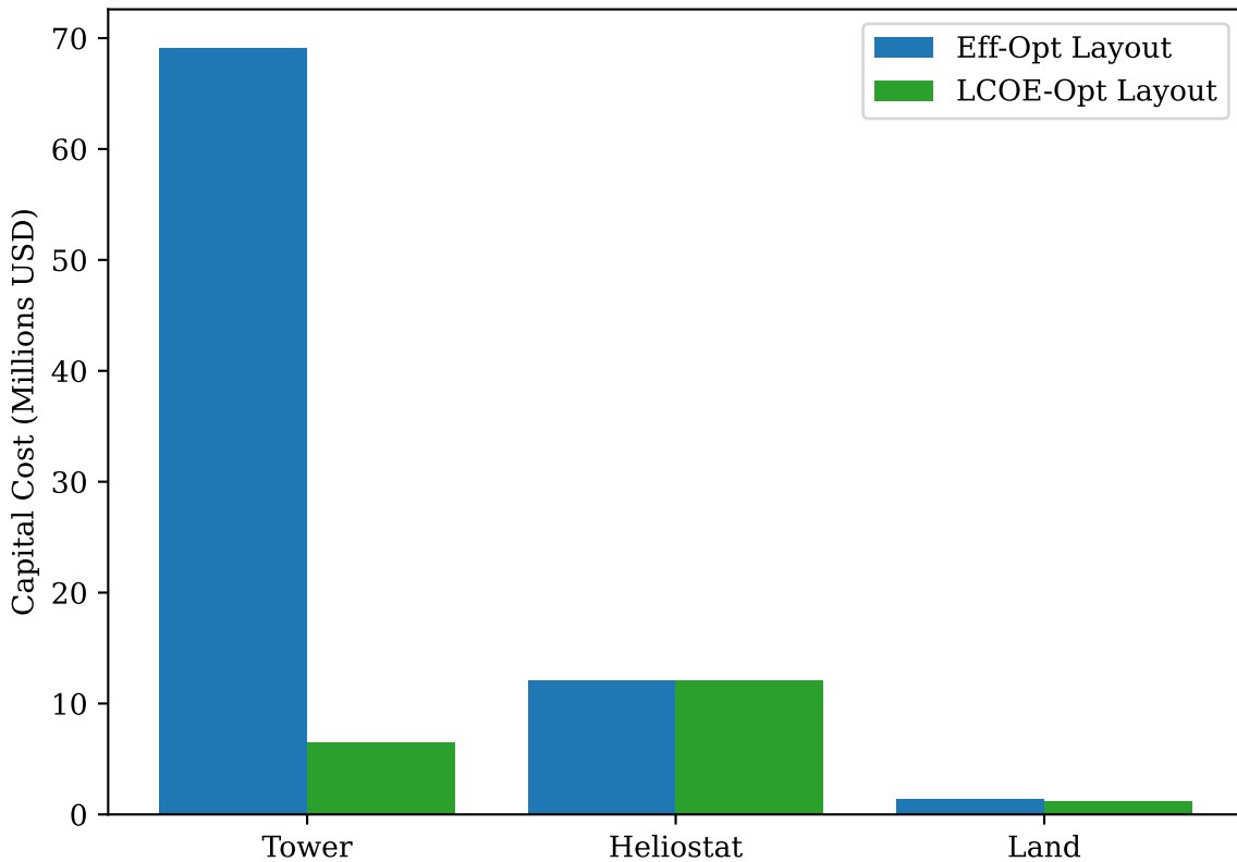
Capital Cost Breakdown Comparison
