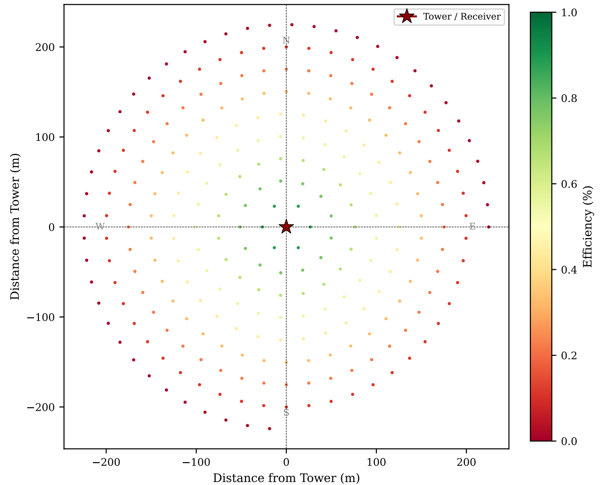
GA-opt LCOE Radial Staggered TH=53.2m, LH=15.74m×19.00m, N=269
