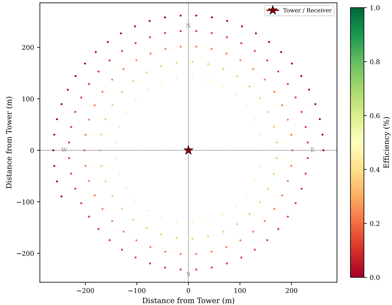
GA-opt Efficiency Radial Staggered TH=283.3m, LH=18.60m×23.46m, N=185
