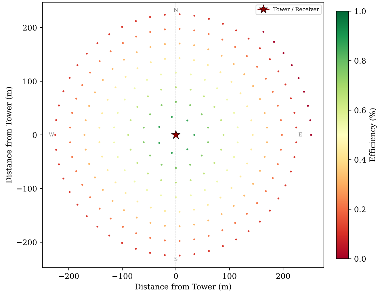
ML-GA LCOE-opt Radial TH=68.7m, LH=14.43m, N=244
