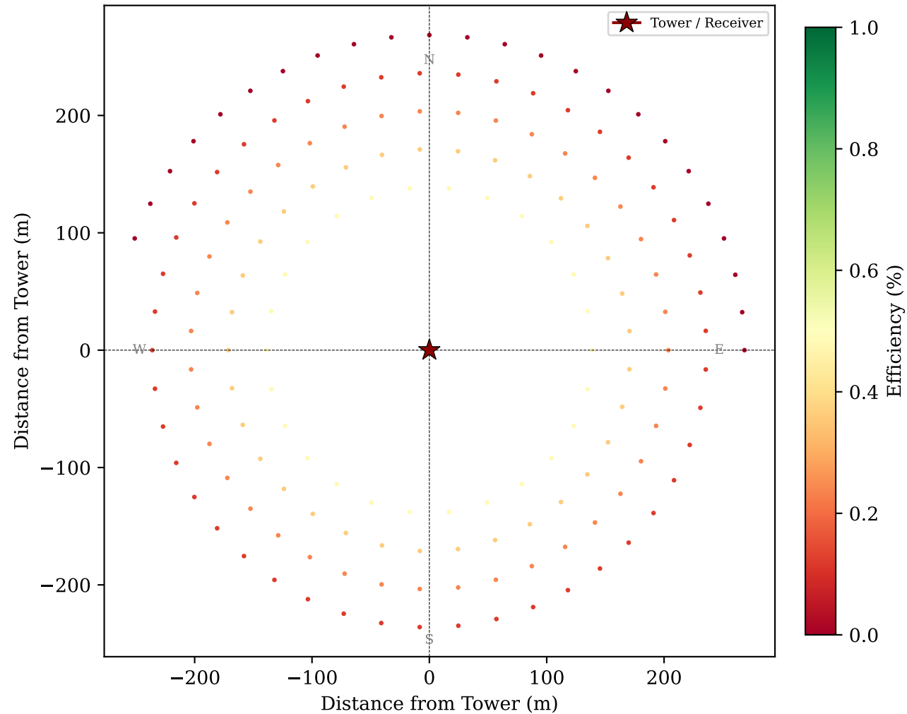
ML-GA Eff-opt Radial TH=277.7m, LH=18.50m, N=167
