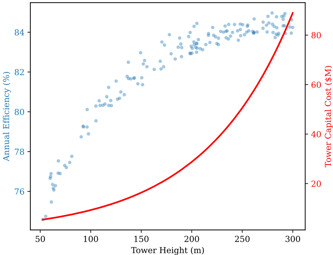
Tower Height Impact on Efficiency and Cost
