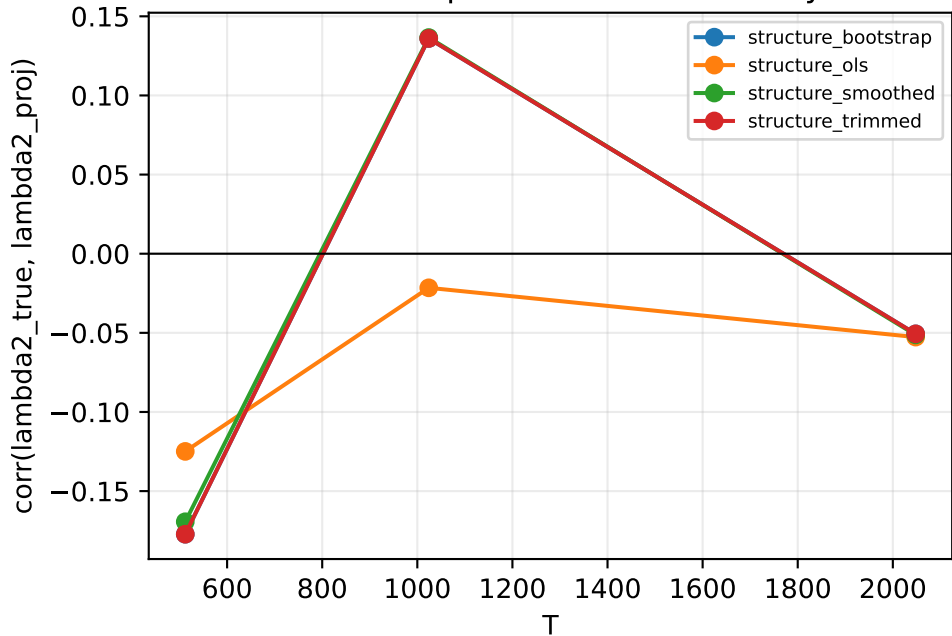
Finite-Sample Curvature Recovery
