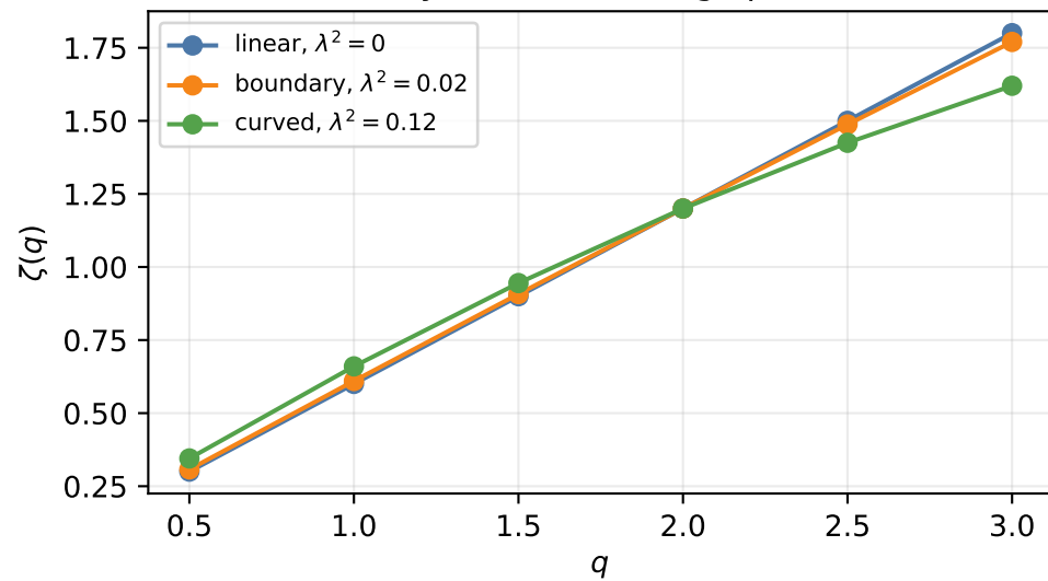
Analytic MRW scaling spectra
