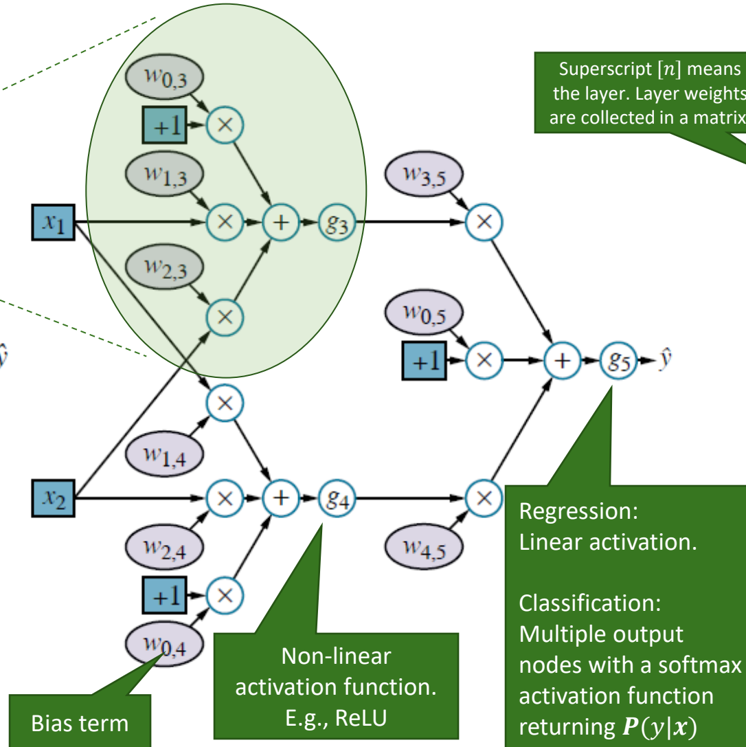
Computational graph
