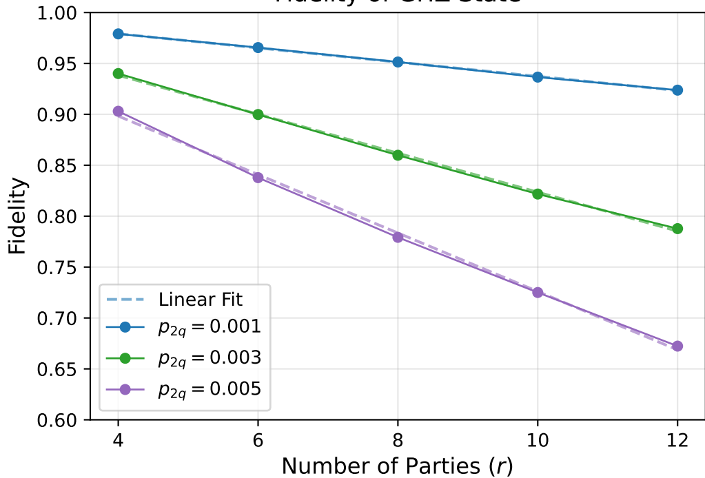
Fidelity of GHZ State
