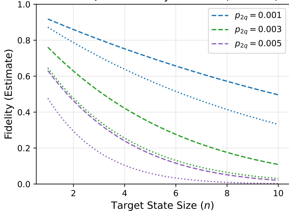
Overall QRACD Fidelity Estimate (Teledata)
