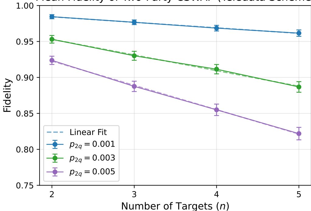
Mean Fidelity of Two-Party CSWAP (Teledata Scheme)
