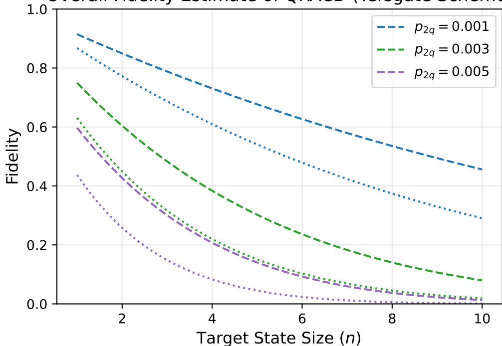
Overall Fidelity Estimate of QRACD (Telegate Scheme)
