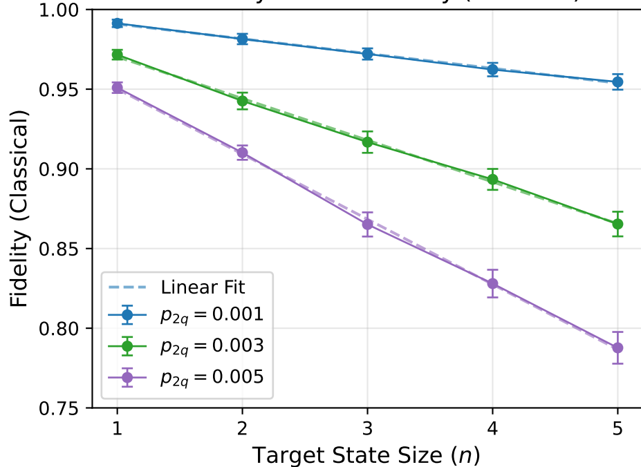
Two-Party CSWAP Fidelity (Teledata)
