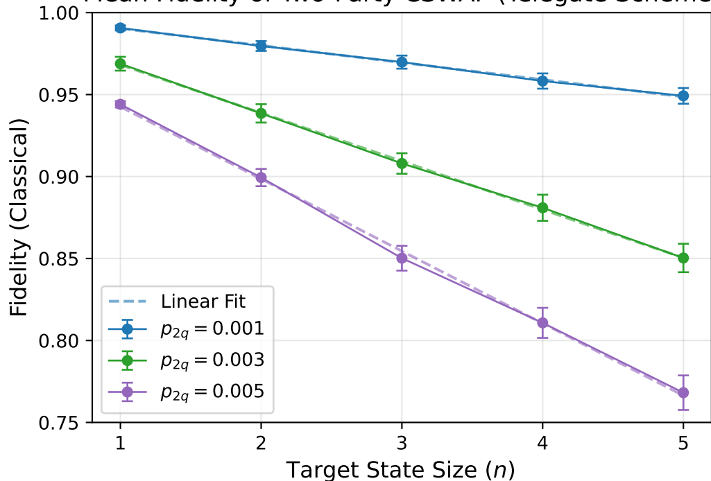
Mean Fidelity of Two-Party CSWAP (Telegate Scheme)
