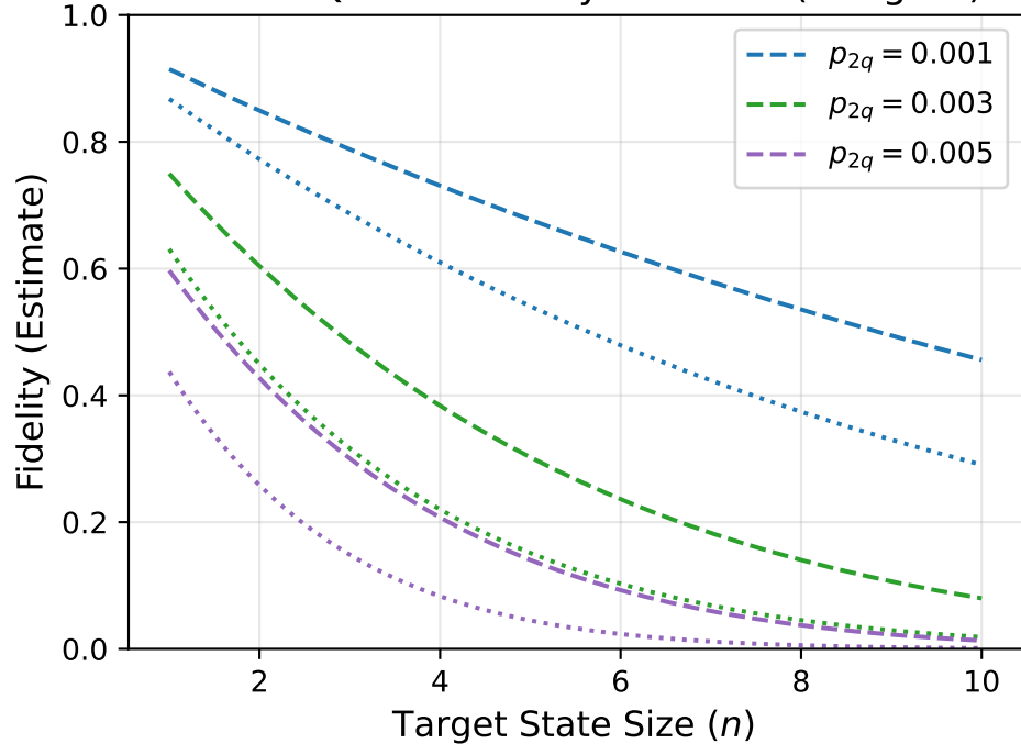
Overall QRACD Fidelity Estimate (Telegate)
