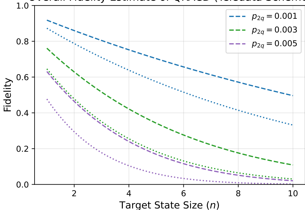
Overall Fidelity Estimate of QRACD (Teledata Scheme)
