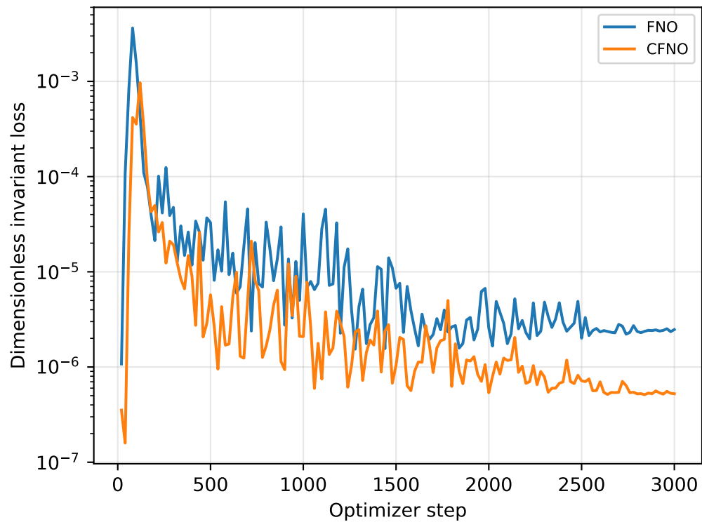
Validation conservation
