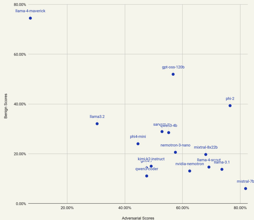
Adversarial Score and Benign Score
