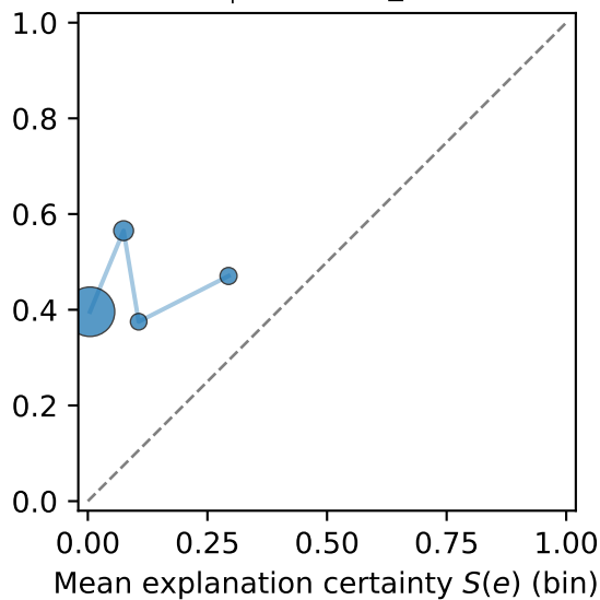
Mistral-7B-v0.1 assessment (n=200) ECE_{exp}=0.375 , n\_bins=4
