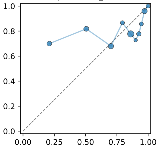
Qwen2.5-7B-Instruct assessment (n=200) ECE_{exp}=0.137 , n\_bins=10
