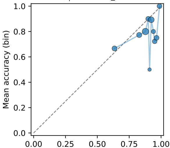
Qwen2.5-7B-Instruct justificatory (n=200) ECE_{exp}=0.085 , n\_bins=10
