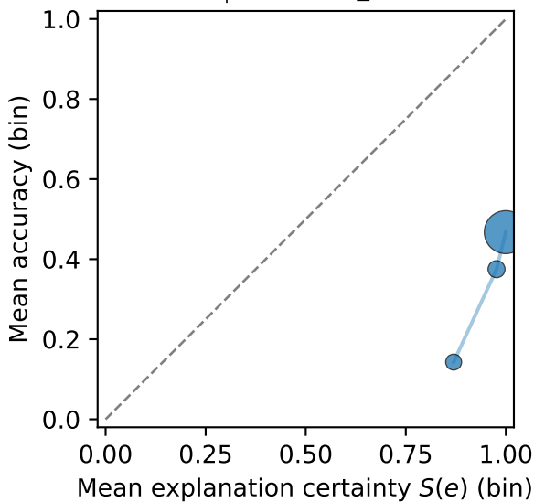
Mistral-7B-v0.1 justificatory (n=199) ECE_{exp}=0.561 , n\_bins=3
