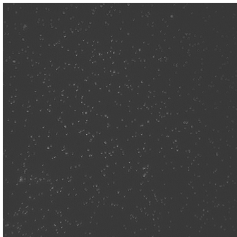
\hat{\mathcal{S}}_{\text{avg}}
