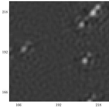
\hat{\mathcal{S}}_{\text{CC}}
