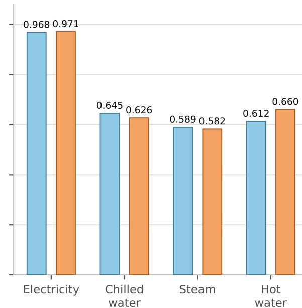
K=100 buildings
