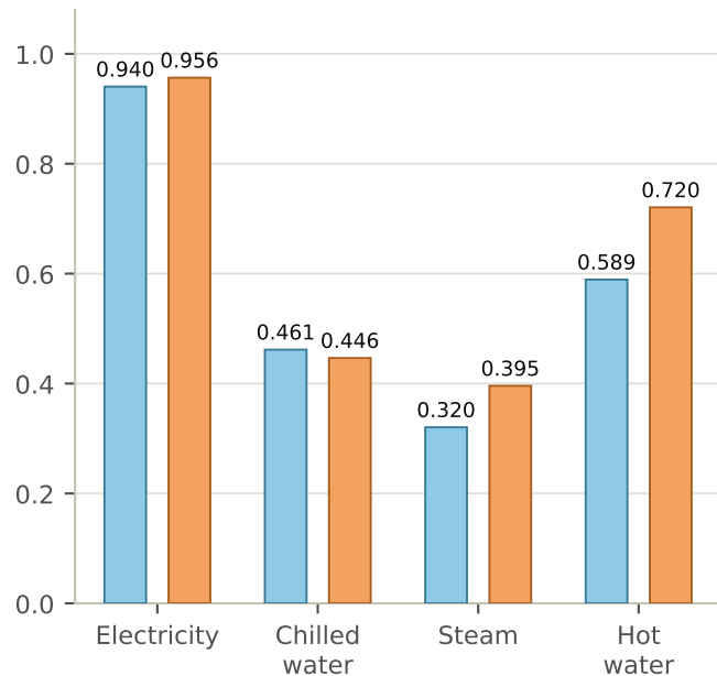
K=10 buildings
