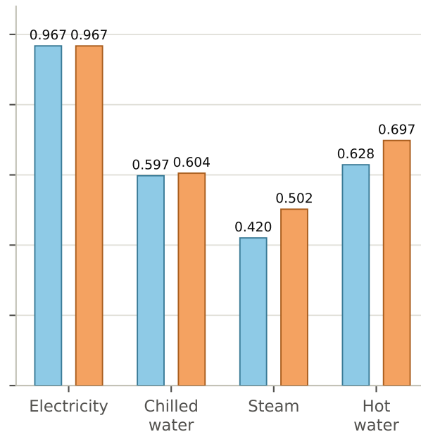
K=50 buildings
