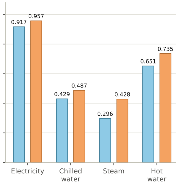
K=20 buildings
