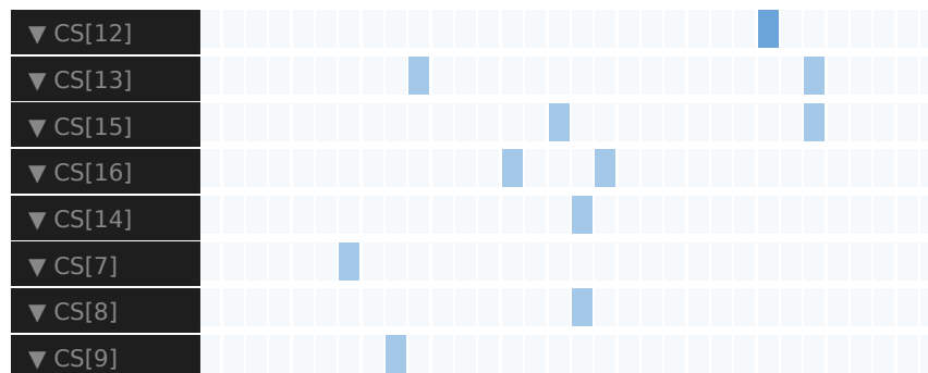
Figure 9: Migration heatmap Level 2: per-task sub-bins within the selected time window
