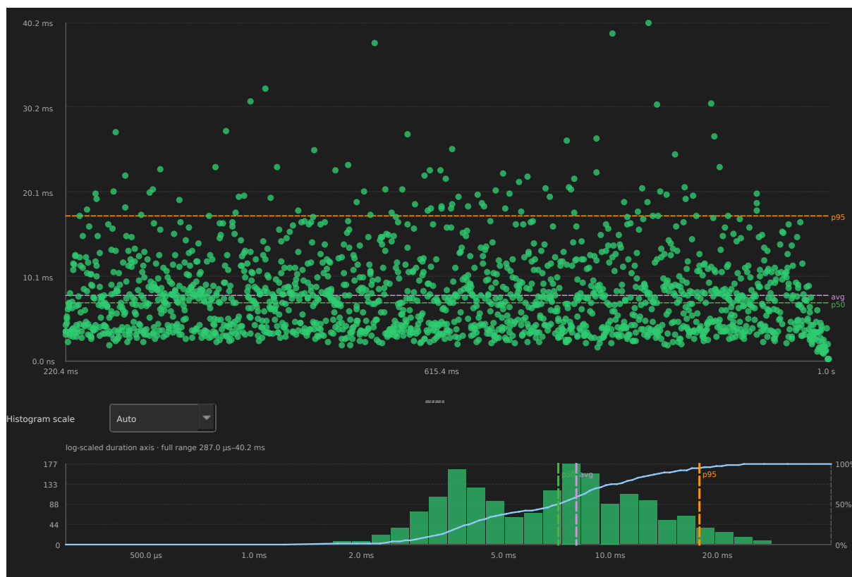
Figure 9: Interval duration distribution for interval id 1 in example-8cores.btf
