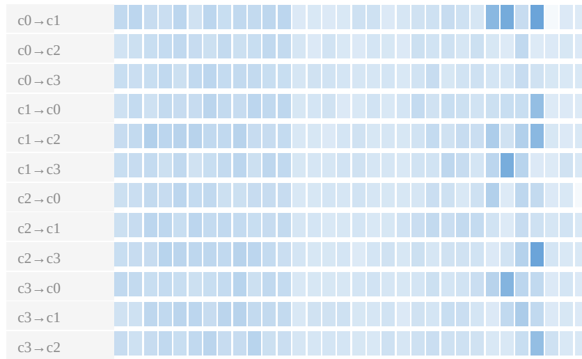
Figure 12: Migration heatmap Level 1: core-pair rows and time bins for example-4cores.btf
