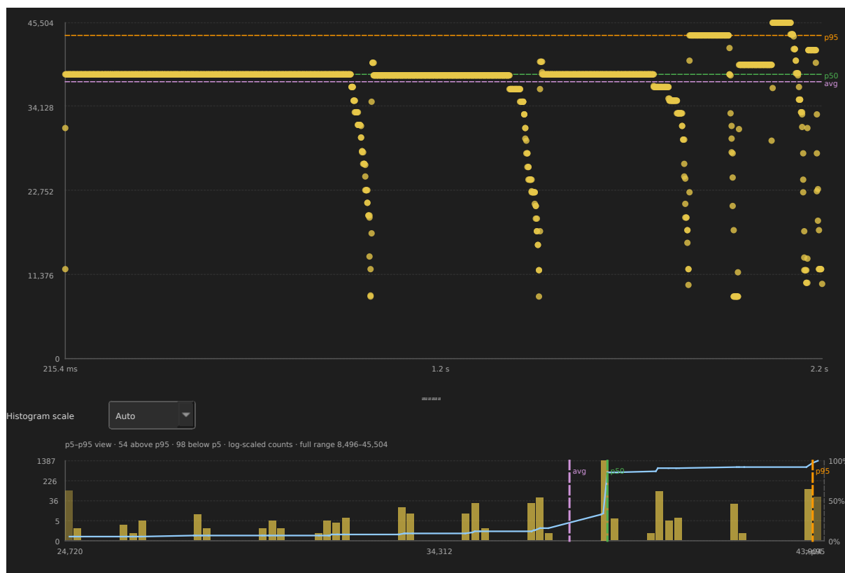
Figure 11: Tag value distribution chart for tag0_event in example-8cores.btf
