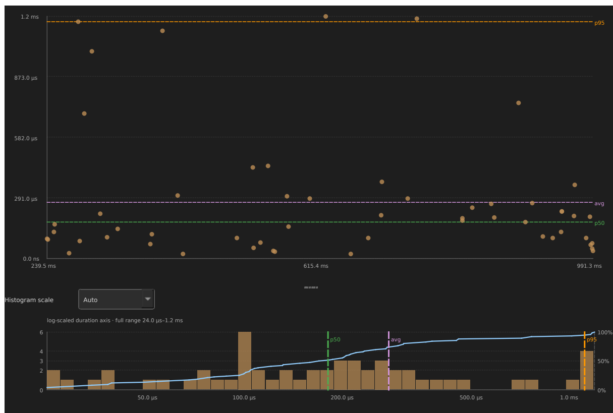
Figure 6: Preemption chain distribution CS[24] preempted by CS[25] in example-8cores.btf
