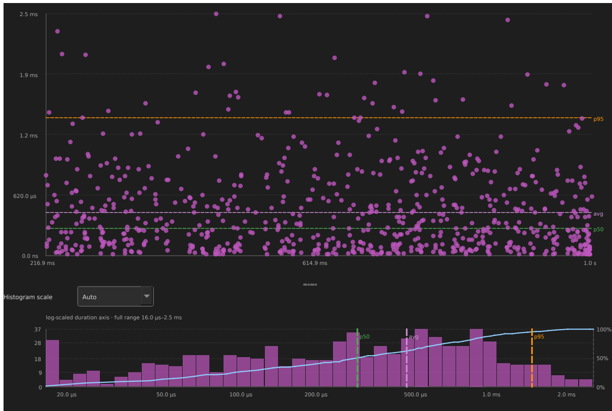
Figure 3: Execution time distribution for CS[11] in example-8cores.btf
