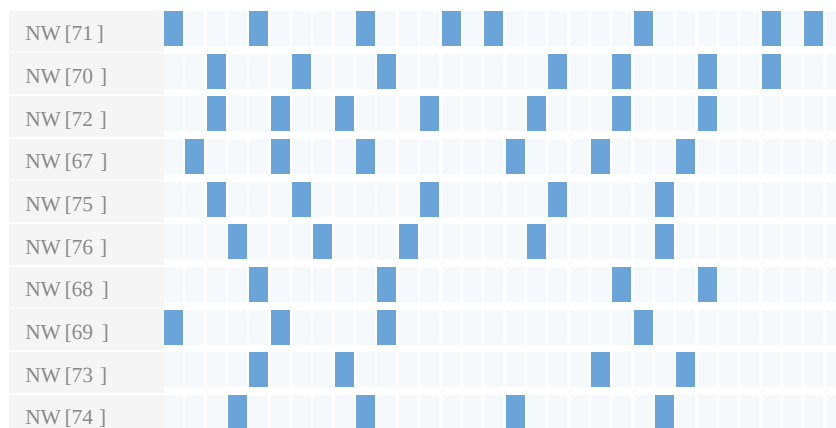
Figure 13: Migration heatmap Level 2: per-task sub-bins after drilling from example-4cores.btf
