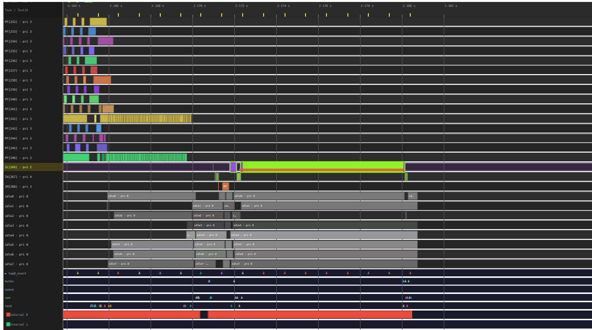
Figure 7: Timeline view: IL[266] with red priority-inheritance stripe (example-8cores.btf)
