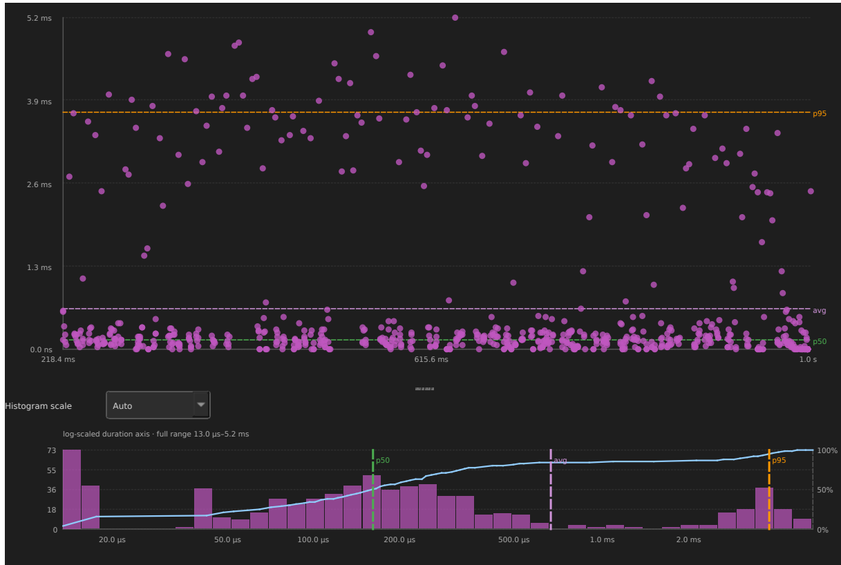
Figure 4: Blocking time distribution for CS[11] in example-8cores.btf
