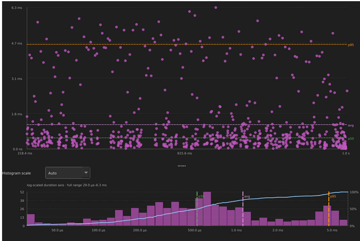
Figure 5: Inter-arrival time distribution for CS[11] in example-8cores.btf
