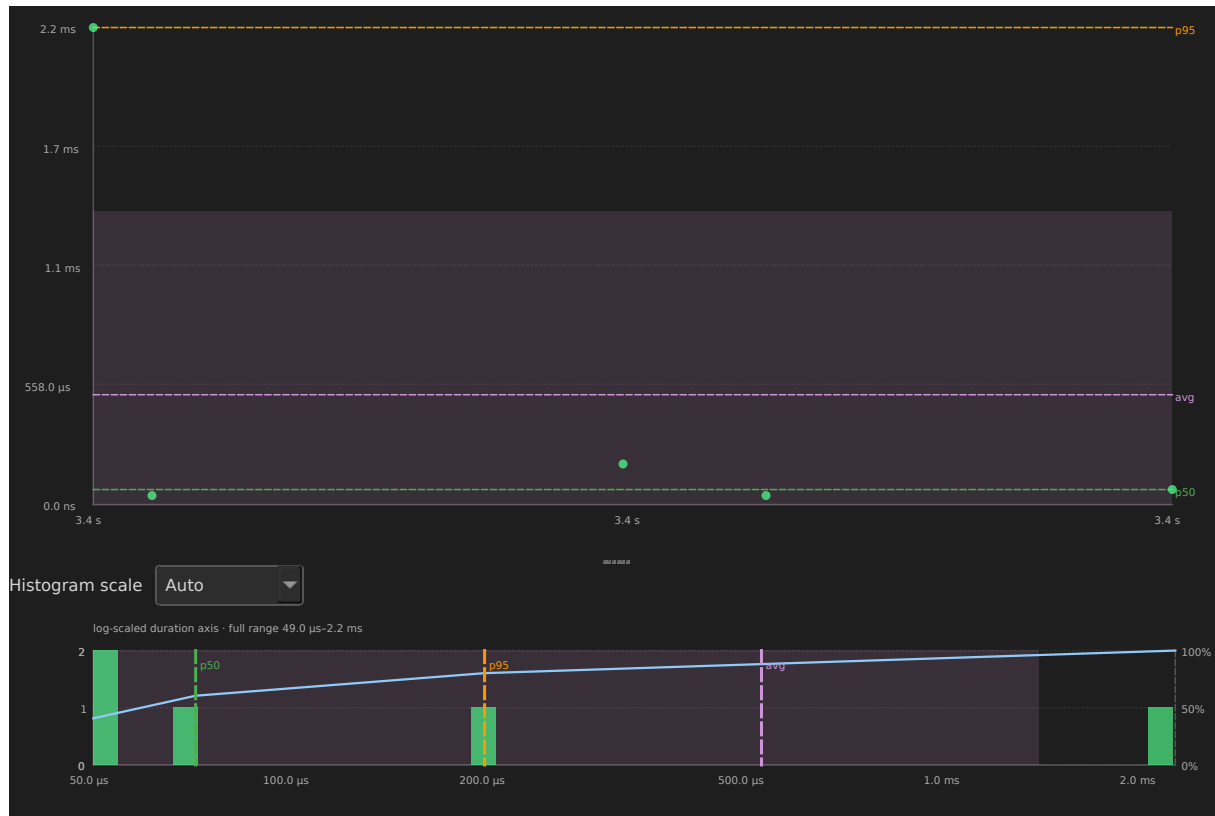
Figure 10: Dispatch latency distribution for SR0[271] in example-8cores.btf.gz
