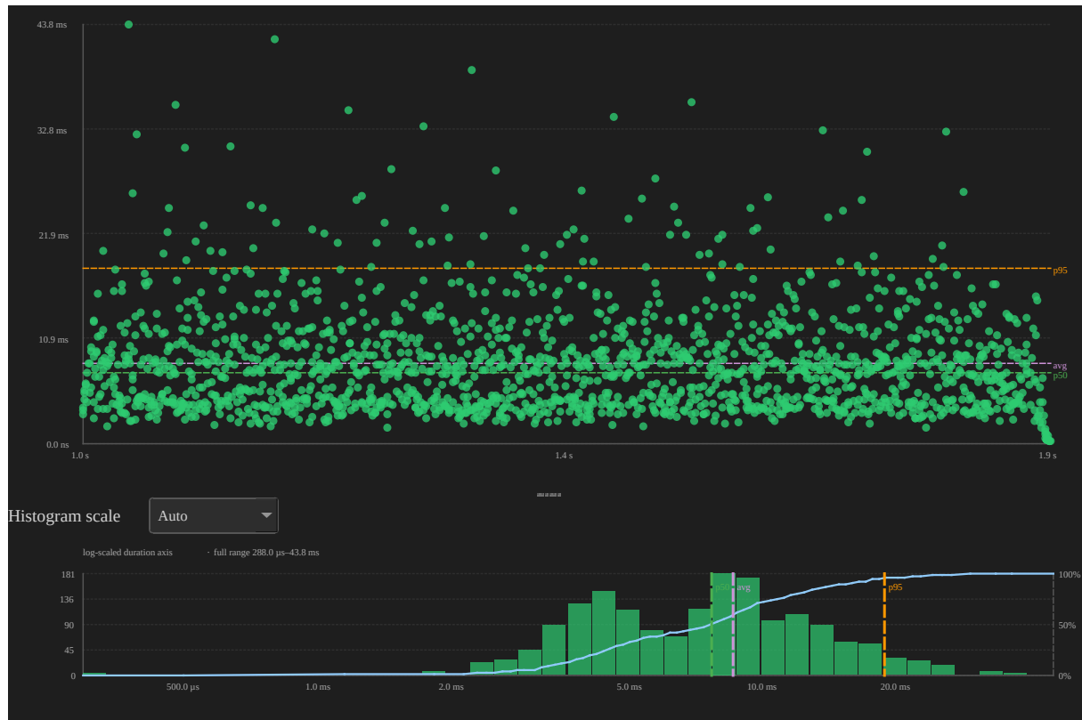
Figure 20: Interval duration distribution for interval id 1 in example-8cores.btf.gz
