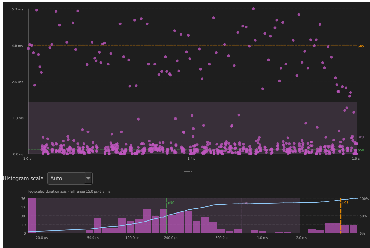
Figure 9: Blocking time distribution for CS[11] in example-8cores.btf.gz
