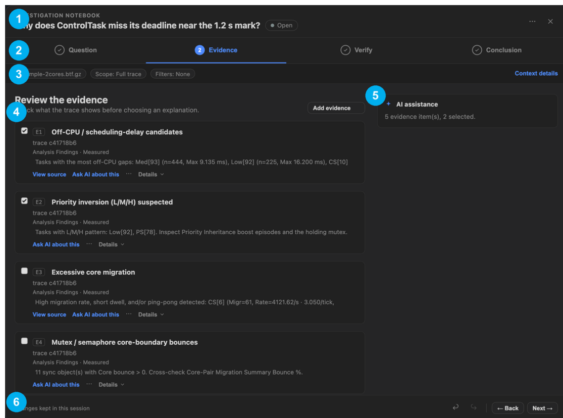
Figure 6: Investigation Notebook — Evidence step
