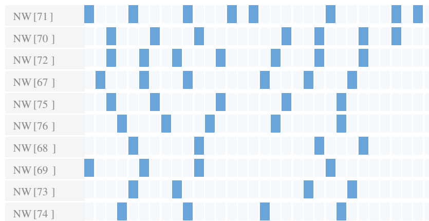
Figure 11: Migration heatmap Level 2: per-task sub-bins after drilling from example-4cores.btf
