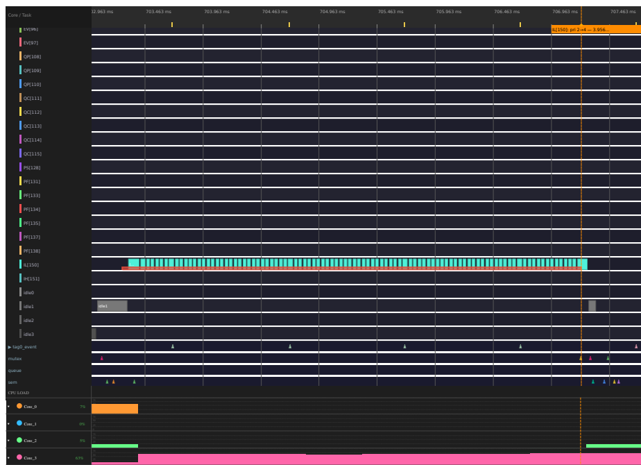
Figure 7: Timeline core view: IL[150] on Core_3 with red priority-inheritance stripe (example-4cores.btf)
