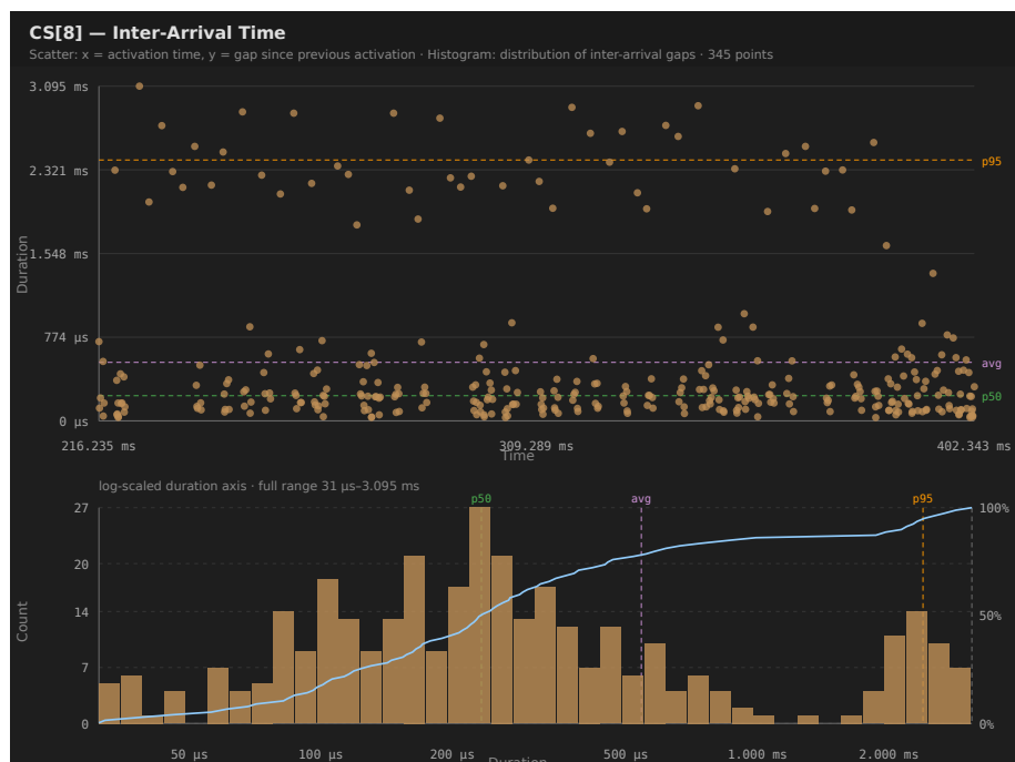
Figure 5: Inter-arrival time distribution for CS[8] in example-4cores.btf
