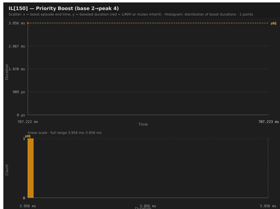
Figure 8: Priority boost distribution chart for IL[150] in example-4cores.btf
