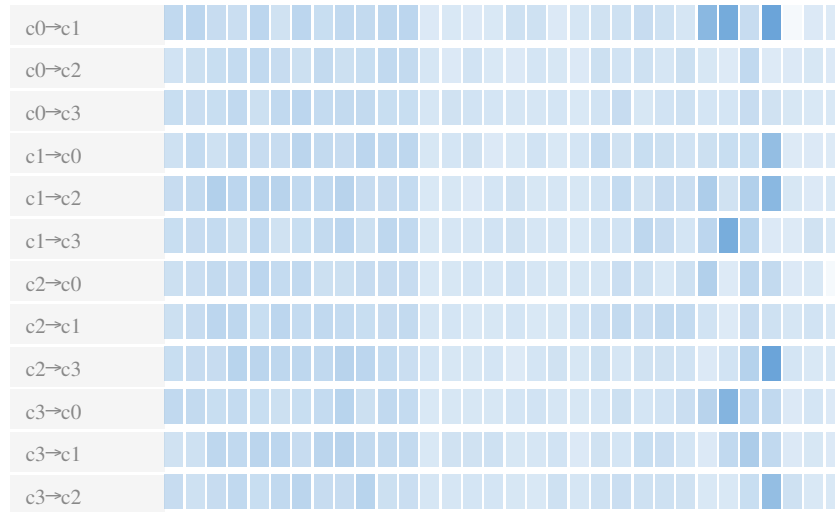
Figure 10: Migration heatmap Level 1: core-pair rows and time bins for example-4cores.btf
