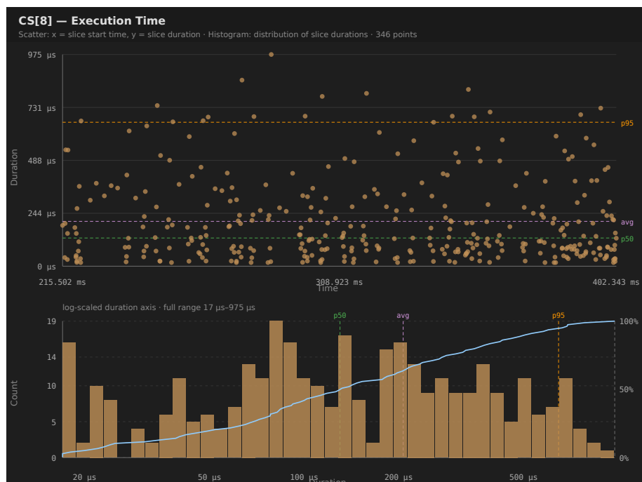
Figure 3: Execution time distribution for CS[8] in example-4cores.btf
