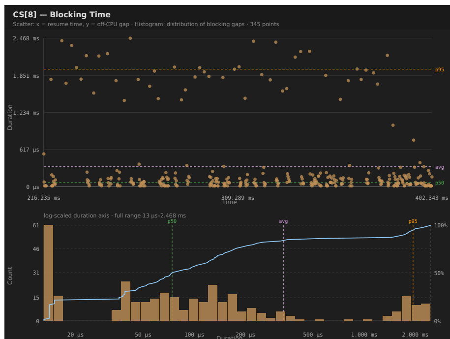
Figure 4: Blocking time distribution for CS[8] in example-4cores.btf
