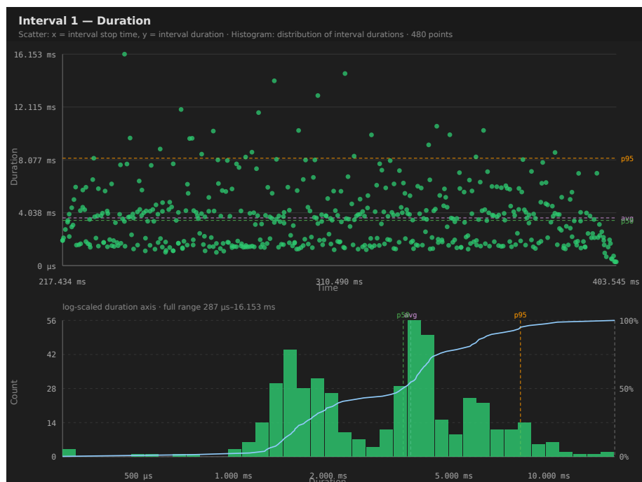
Figure 9: Interval duration distribution for interval id 1 in example-4cores.btf
