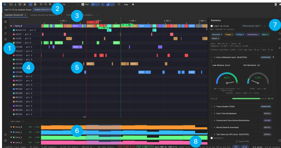
Figure 3: BTFViewer 主視窗
