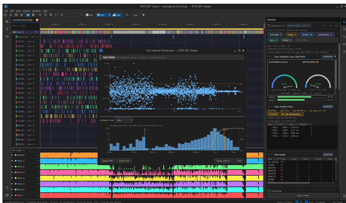
Figure 2: BTFViewer
