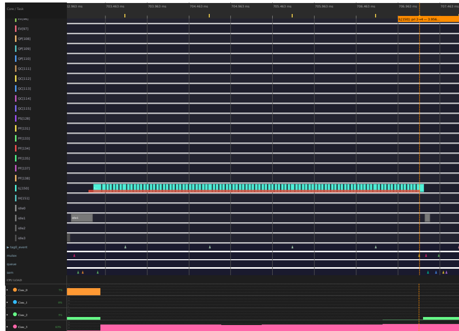
Figure 6: Timeline Core View showing the low-priority mutex holder with a red priority-boost stripe during the mutex inheritance window
