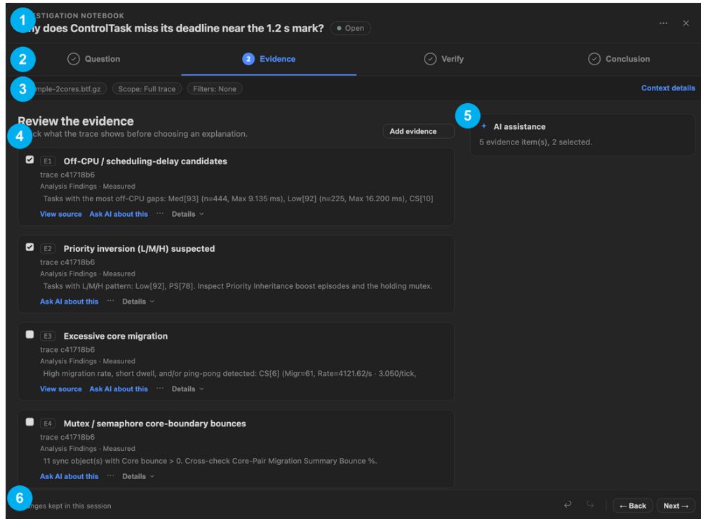
Figure 7: Investigation Notebook —Evidence step
