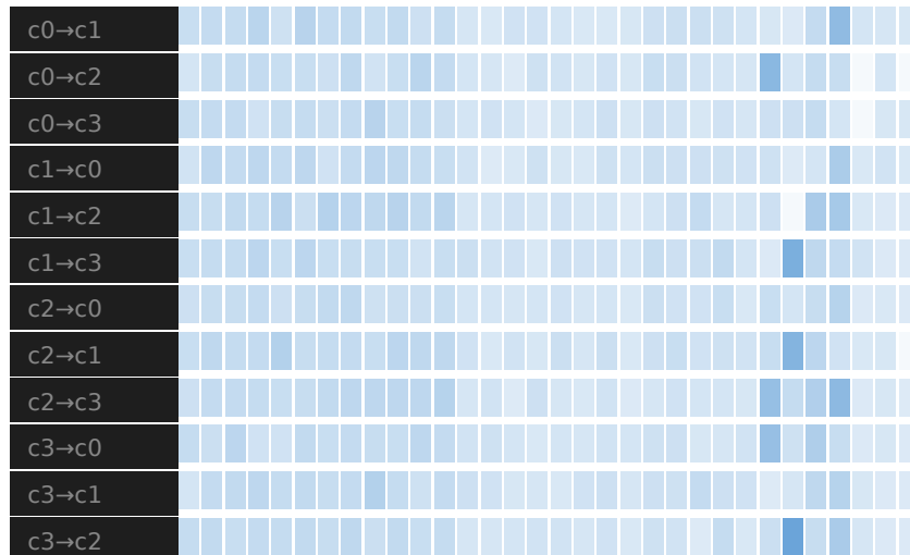
Figure 15: Migration heatmap Level 1: core-pair rows and time bins for example-8cores.btf
