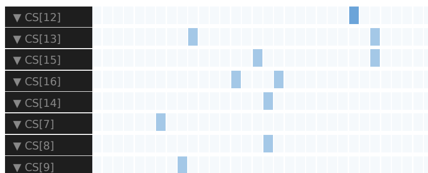
Figure 16: Migration heatmap Level 2: per-task sub-bins after drilling from example-8cores.btf
