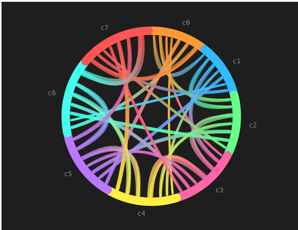
Figure 17: Migration chord diagram: directional core-to-core migration volume for example-8cores.btf
