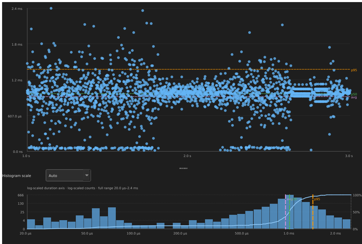
Figure 10: Tick interval distribution chart — scatter and histogram of consecutive TICK gaps in example-8cores.btf
