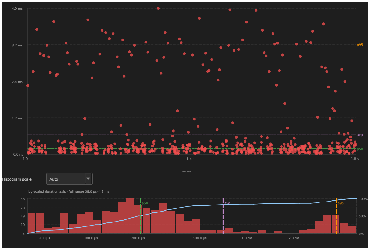
Figure 14: Post-migration gap distribution for CS[22] in example-8cores.btf
