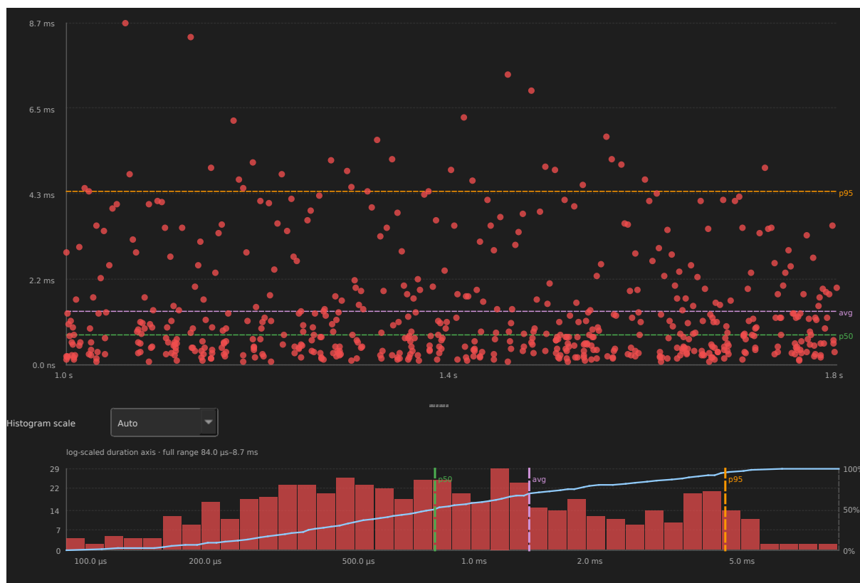
Figure 13: Time between migrations for CS[22] in example-8cores.btf
