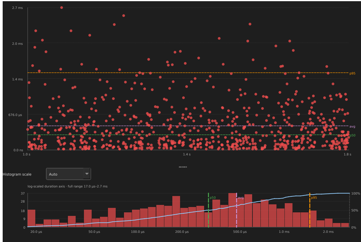
Figure 12: On-core dwell time distribution for CS[22] in example-8cores.btf
