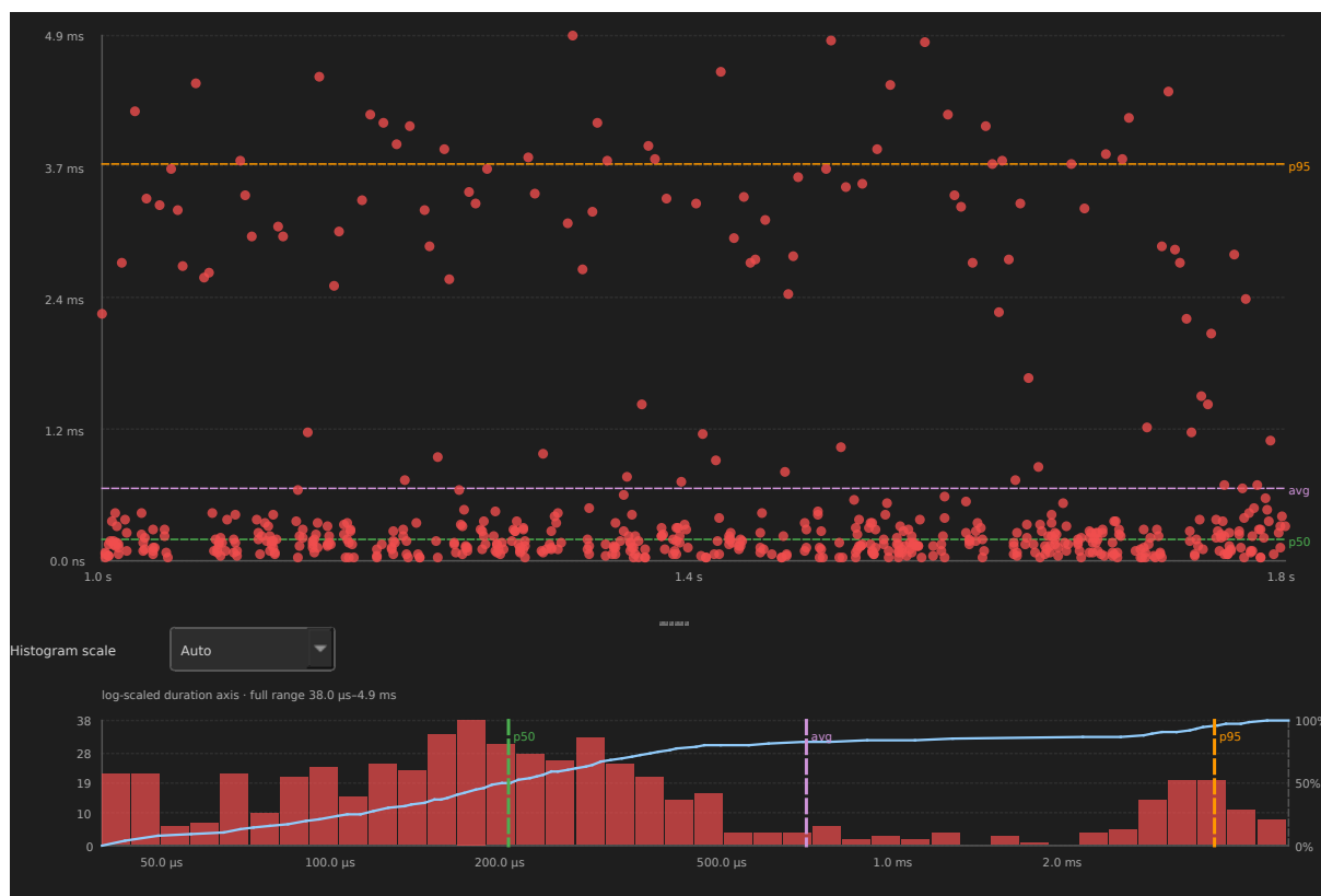
Figure 10: Post-migration gap distribution for CS[22] in example-8cores.btf — Gap tab
