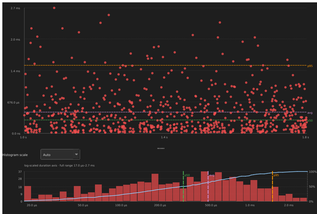
Figure 8: On-core dwell time distribution for CS[22] in example-8cores.btf — Dwell tab
