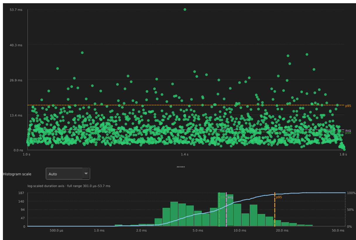
Figure 16: Interval Analysis distribution chart — scatter of start times vs duration, histogram with CDF
