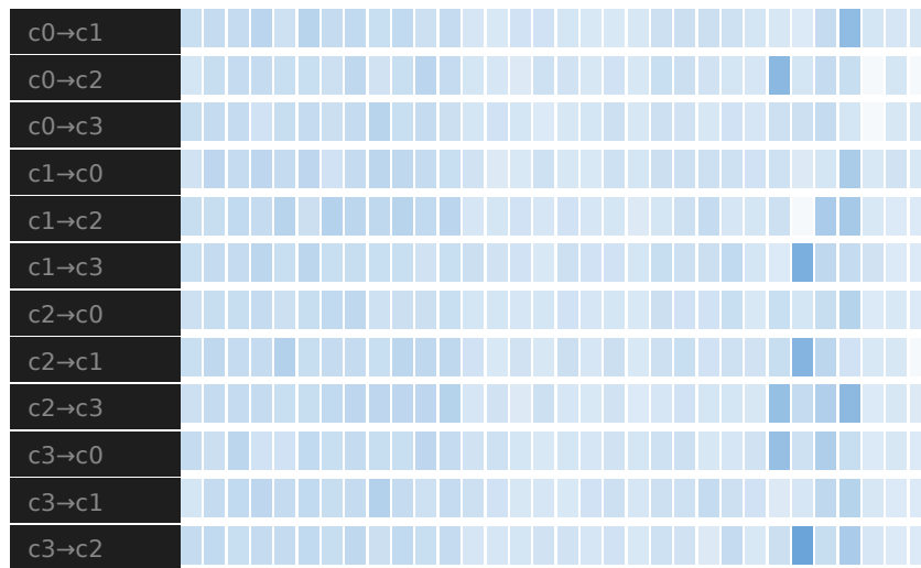
Figure 11: Migration heatmap Level 1: directed core-pair rows and time bins
