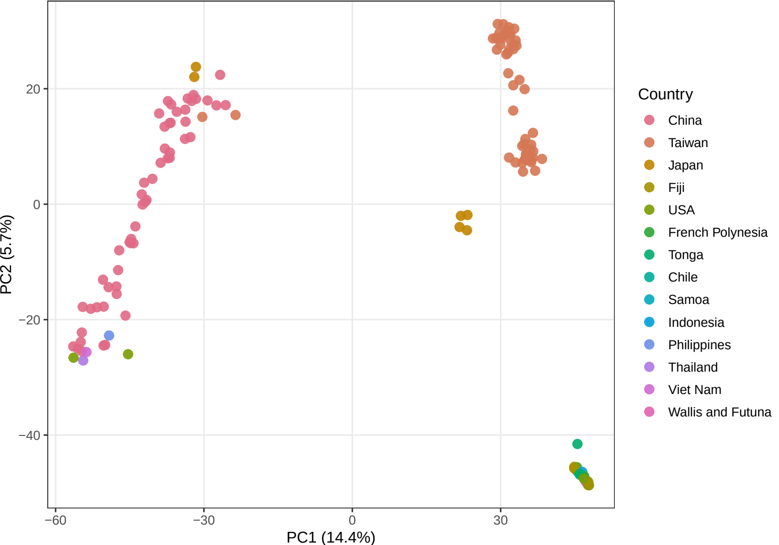
Broussonetia RADseq PCA, site missing <= 40% 85,137 SNPs; 6.33% genotype calls missing before mean imputation
