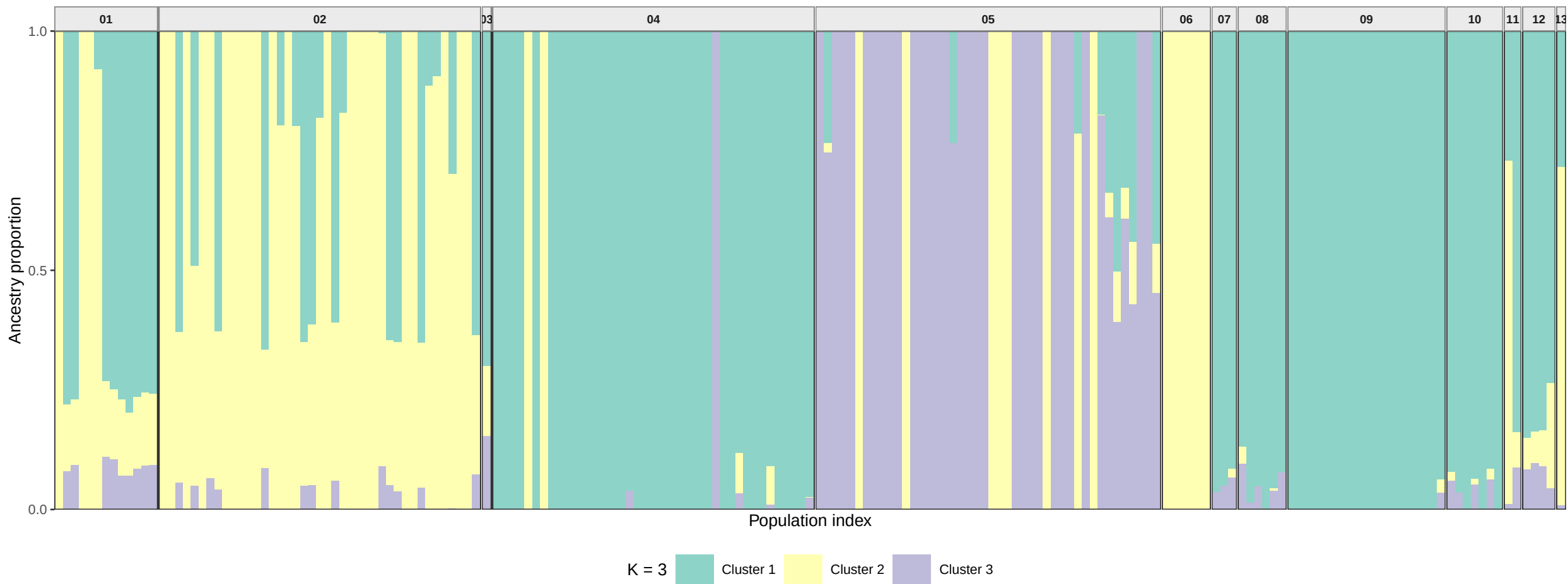
Quercus ADMIXTURE Ancestry Proportions (K = 3)
