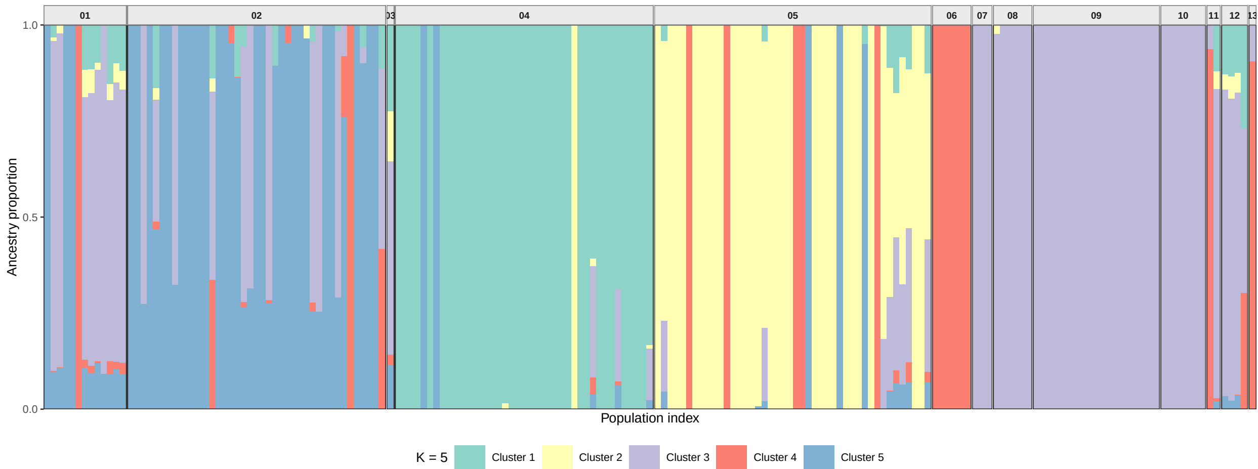
Quercus ADMIXTURE Ancestry Proportions (K = 5)
