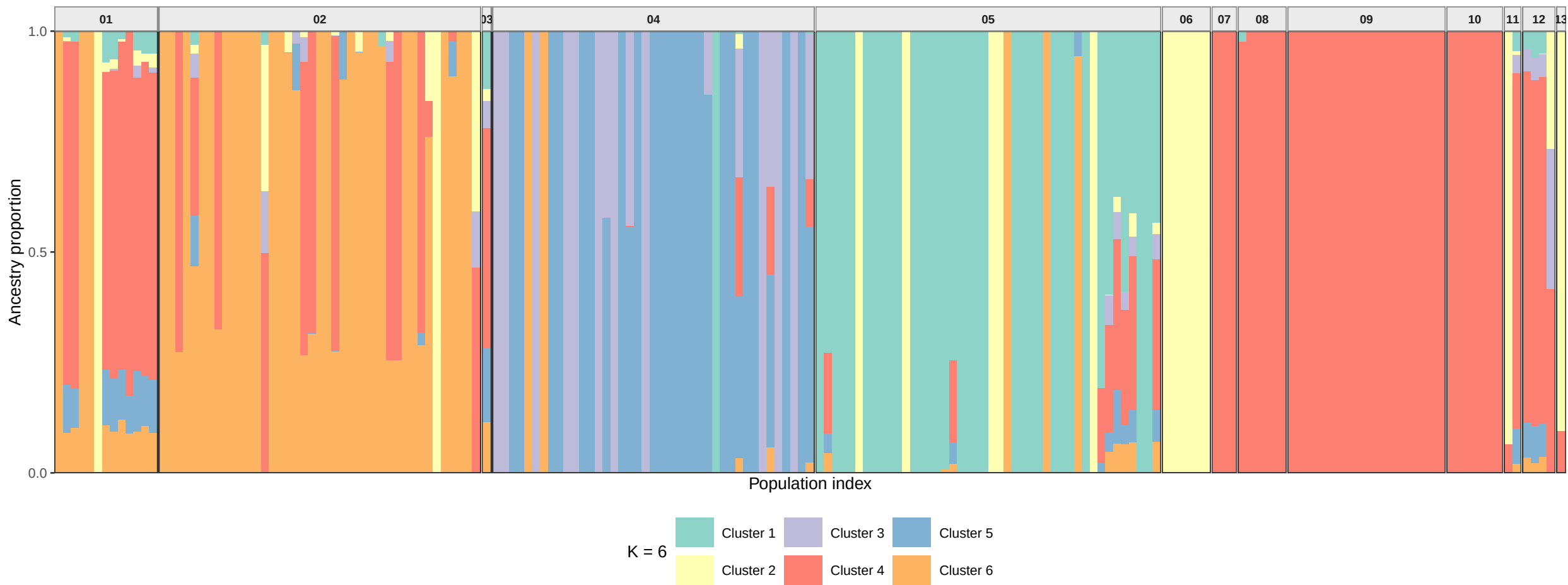
Quercus ADMIXTURE Ancestry Proportions (K = 6)
