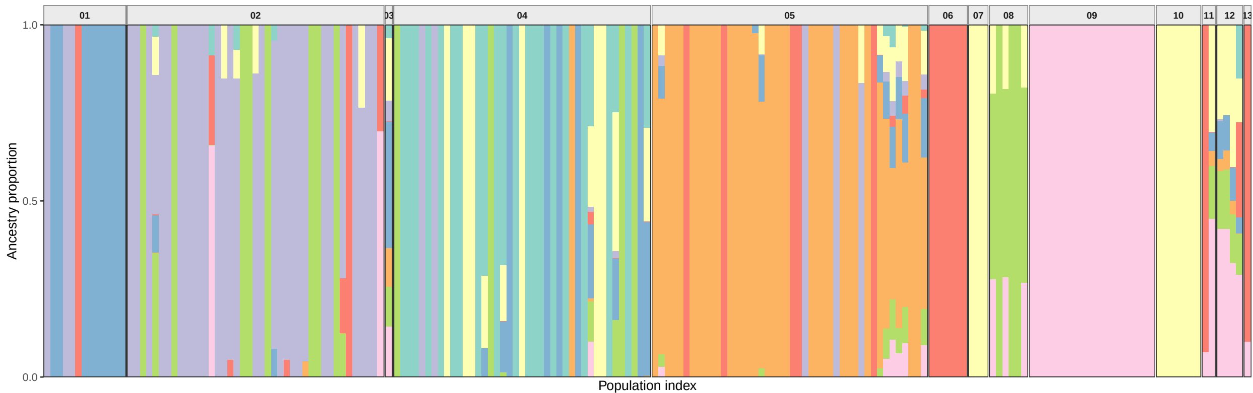
Quercus ADMIXTURE Ancestry Proportions (K = 8)
