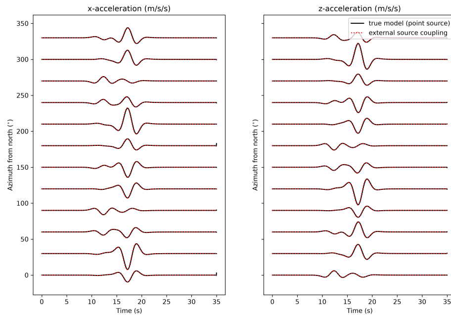
Figure: Comparison of far-field accelerations recorded at the stations indicated in the figure above. To remove numerical high-frequency oscillations, low-pass filter is applied on both cases. It has a good agreement between point source model and coupling model, showing the coupling with external sources works well.
