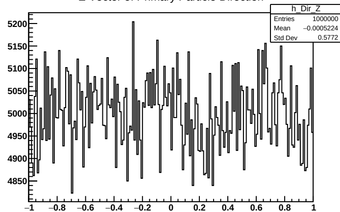
Z Vector of Primary Particle Direction
