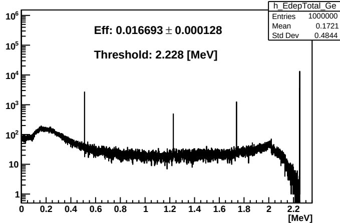
Total Energy Deposit in Ge Crystal [MeV]
