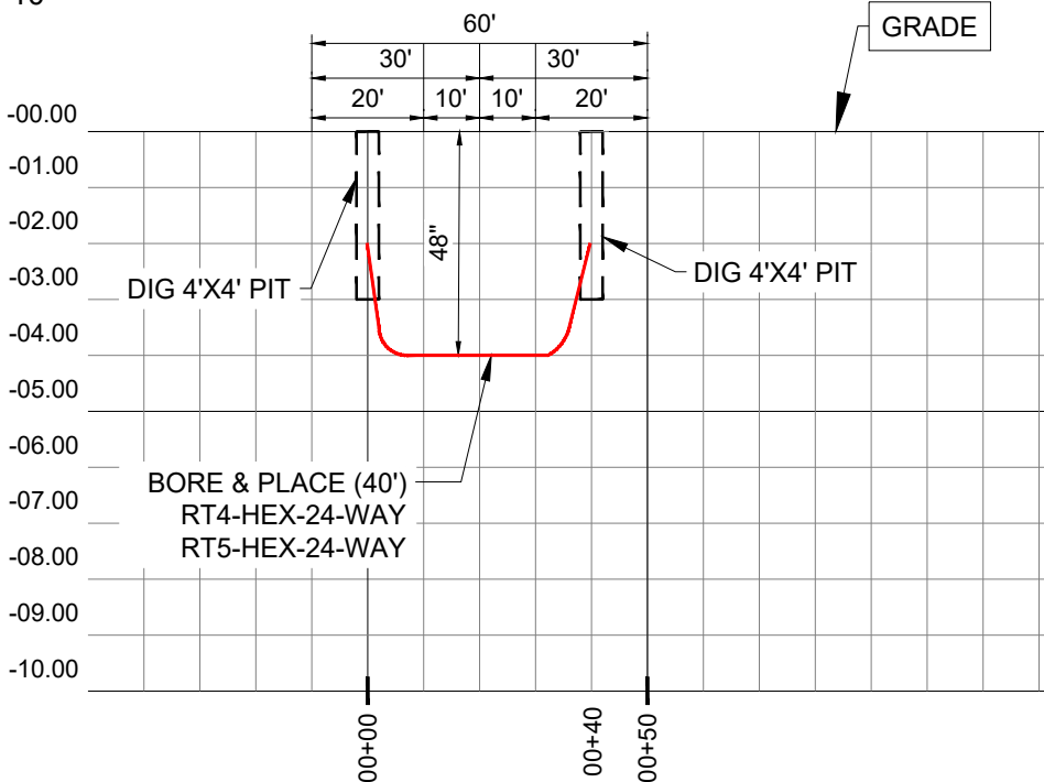
CROSS SECTION VIEW LOOKING EAST (HOLLYHOCK ST)
