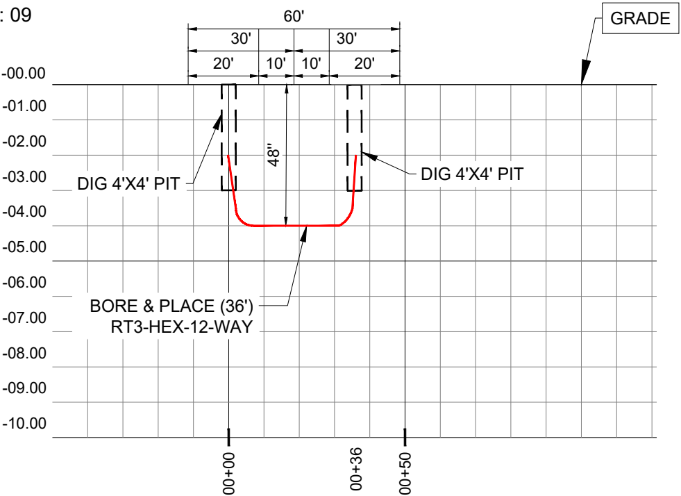
CROSS SECTION VIEW LOOKING WEST (WILTSHIRE AVE)
