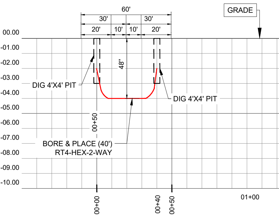
CROSS SECTION VIEW LOOKING SOUTH (LAMPLIGHTER AVE)
