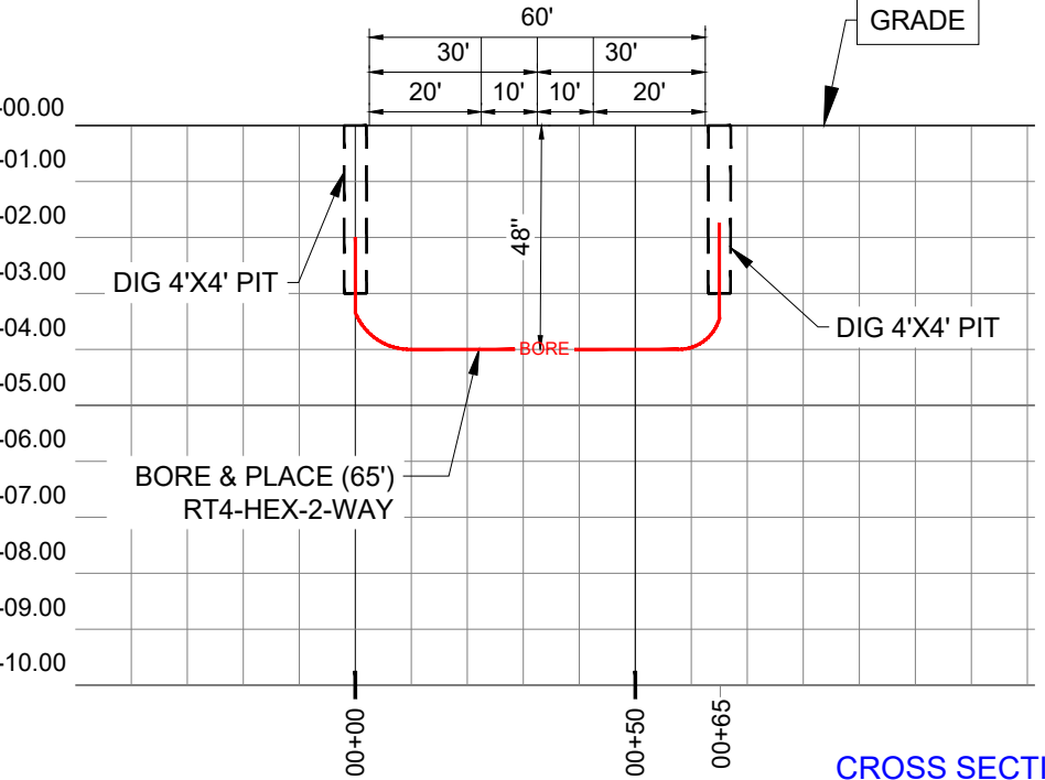
CROSS SECTION VIEW LOOKING SOUTH WEST (LAMPLIGHTER AVE)
