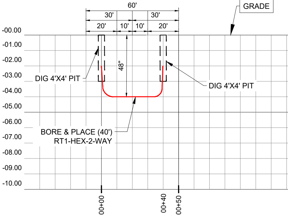
CROSS SECTION VIEW LOOKING WEST (RENTON ST)
