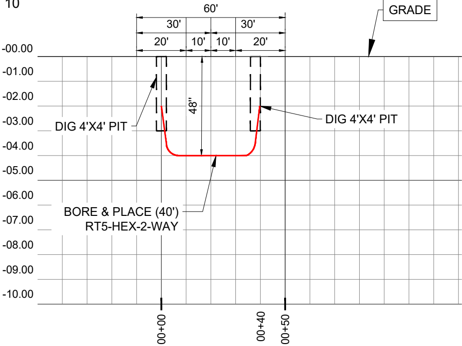
CROSS SECTION VIEW LOOKING WEST (HOLLYHOCK ST)
