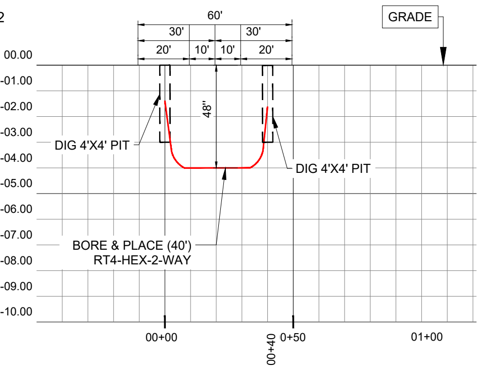
CROSS SECTION VIEW LOOKING WEST (BIRWOOD ST)
