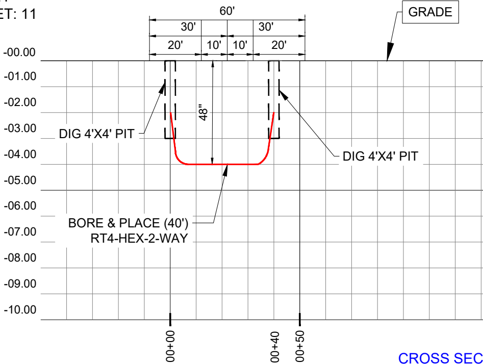
CROSS SECTION VIEW LOOKING SOUTH (LAMPLIGHTER AVE)
