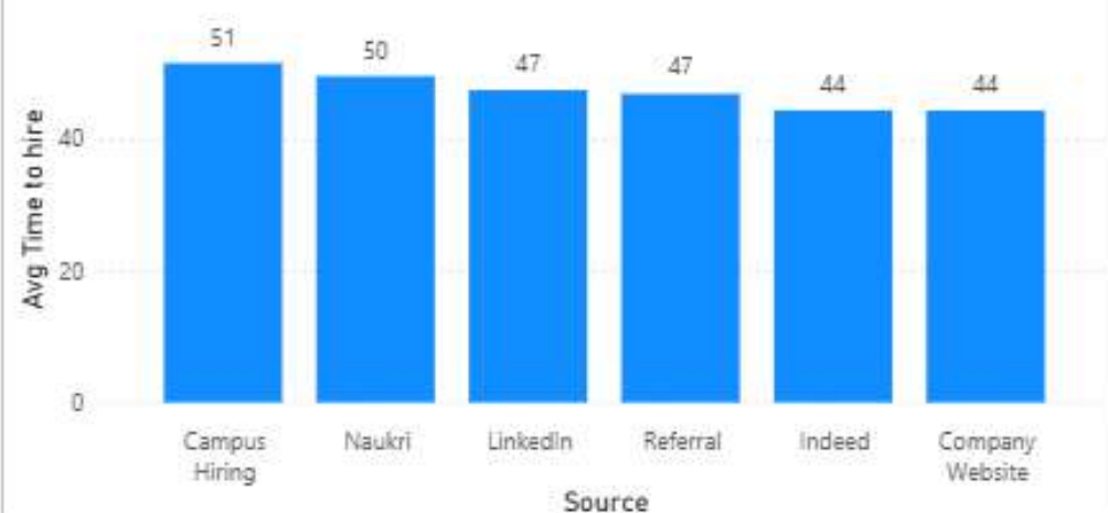
Avg Time to Hire by Source
