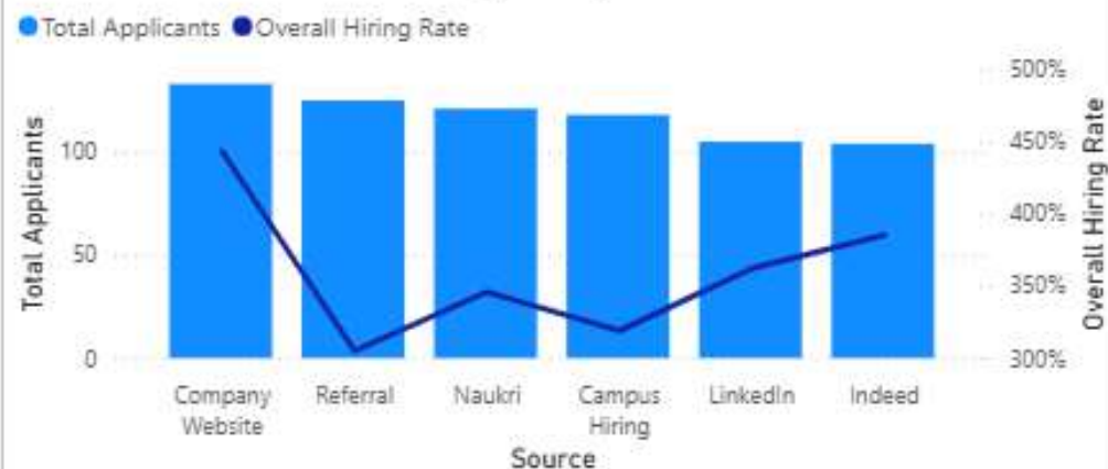
Hiring Rate by Source
