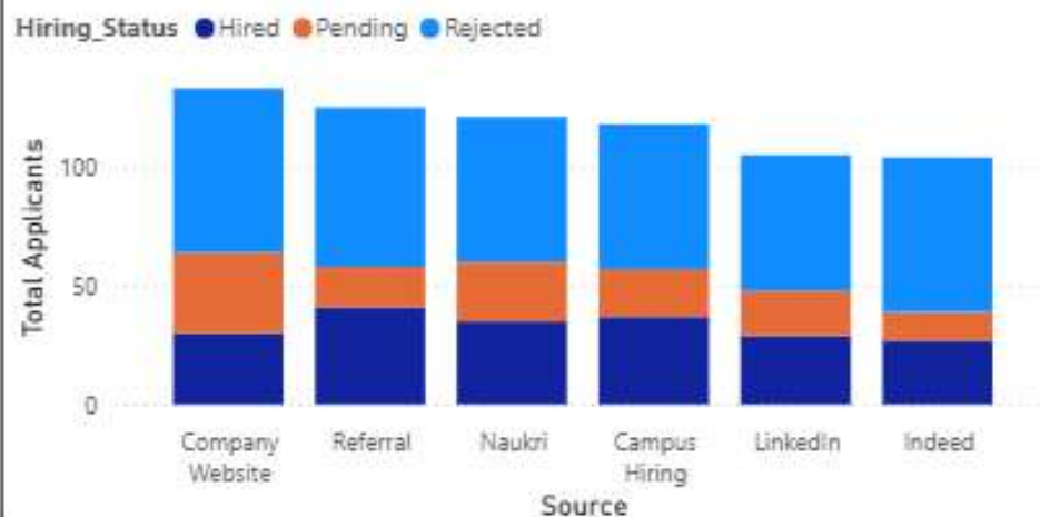
Source X Hiring Status
