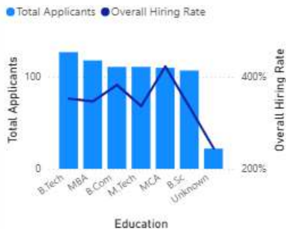
Hiring Rate by Education
