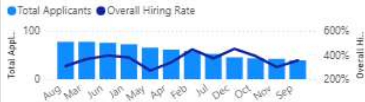
Applications & Hiring Trend
