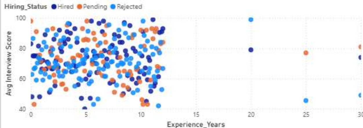
Experience vs Interview Score
