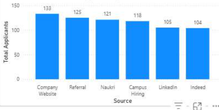
Source X Hiring Status
