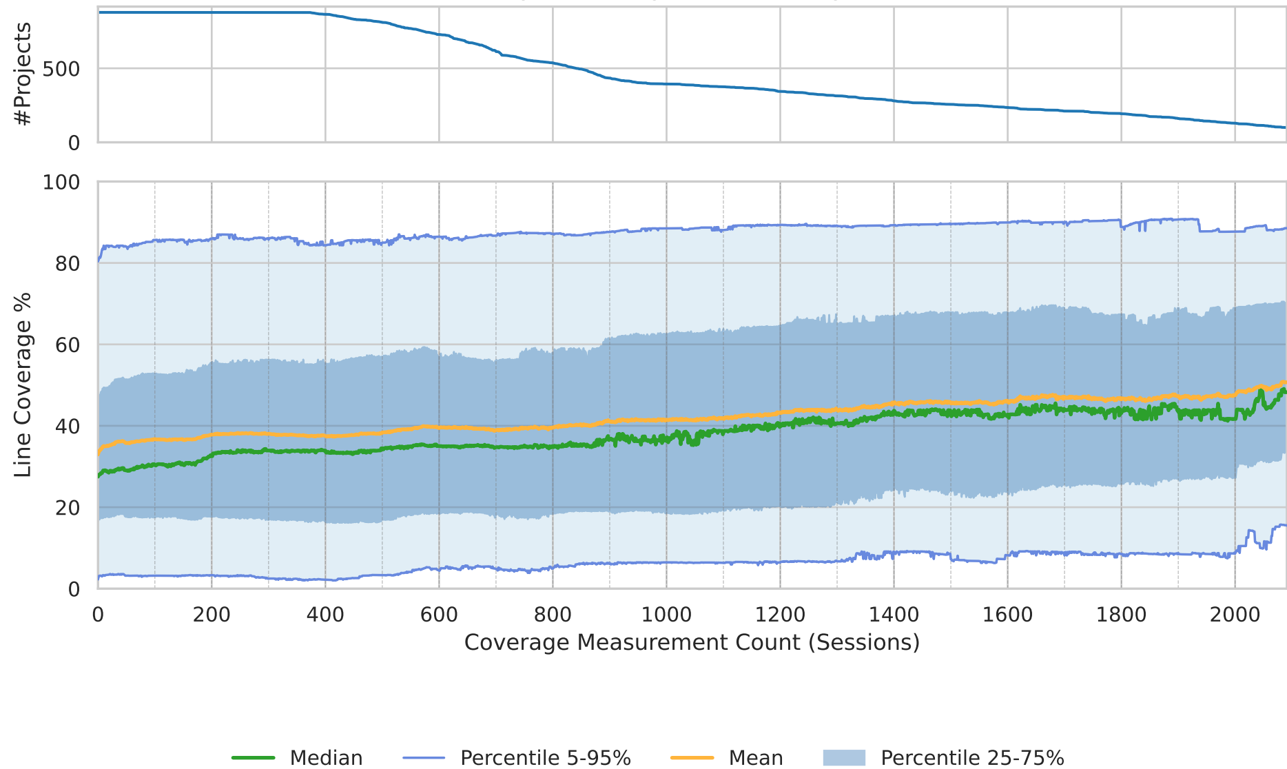
Coverage Percentage across Fuzzing Sessions
