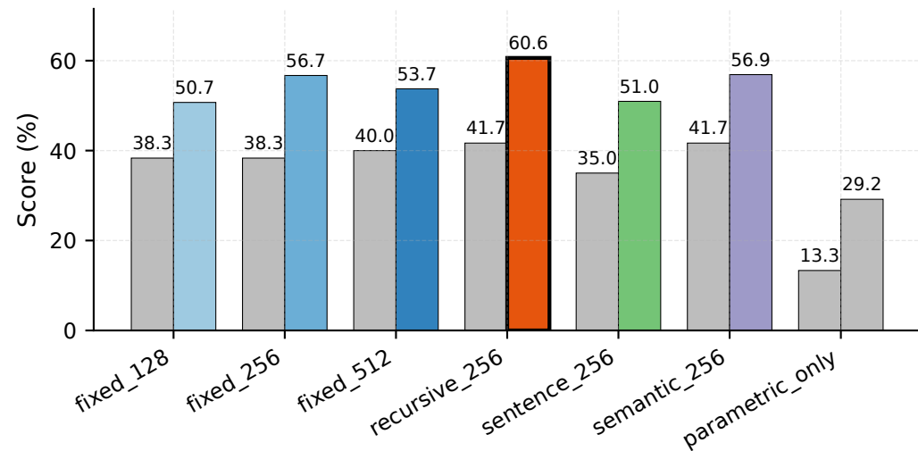
SQuAD v2
