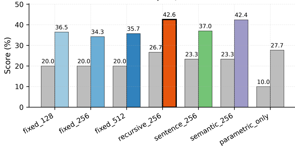
HotpotQA
