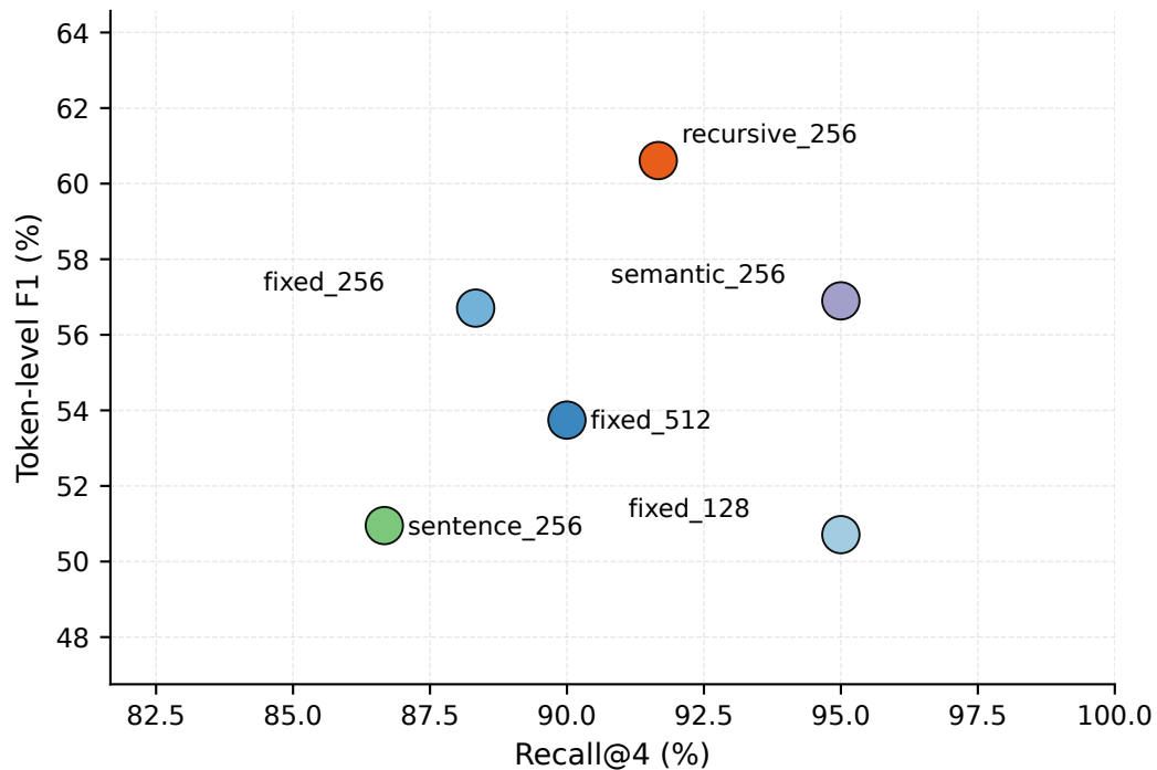
SQuAD v2
