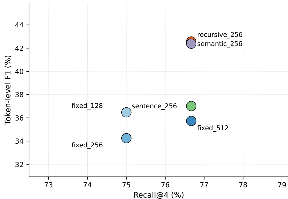
HotpotQA
