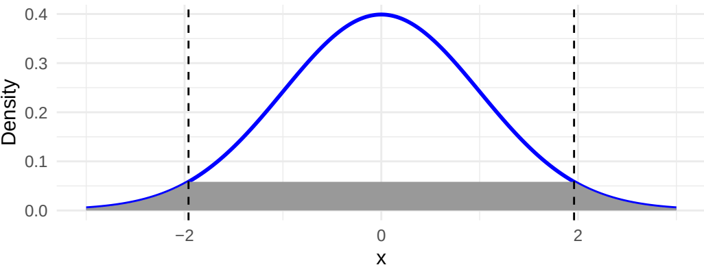
Normal Density Curve with Rejection Area
