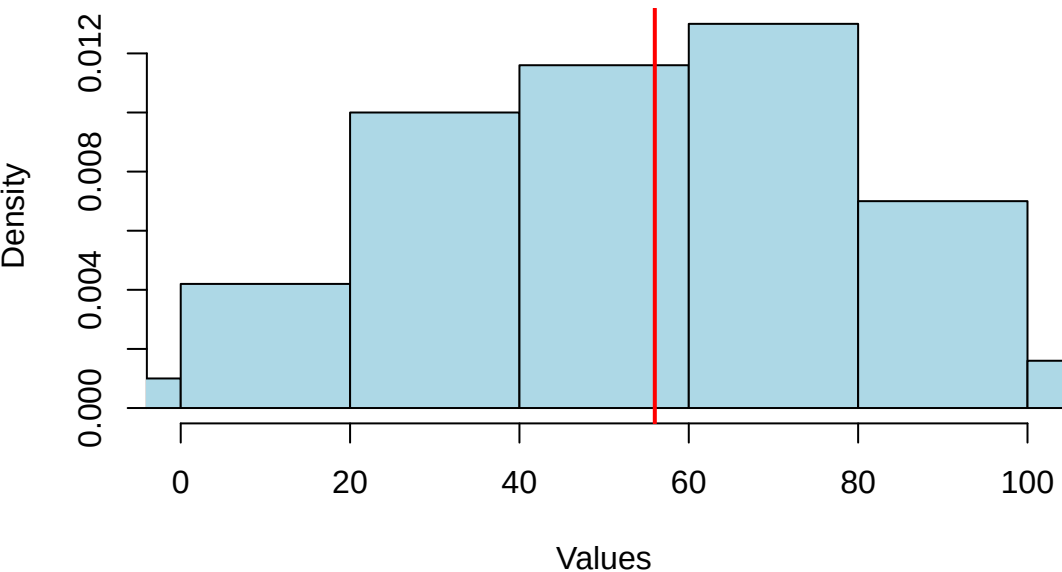
Histogram of Fake Data
