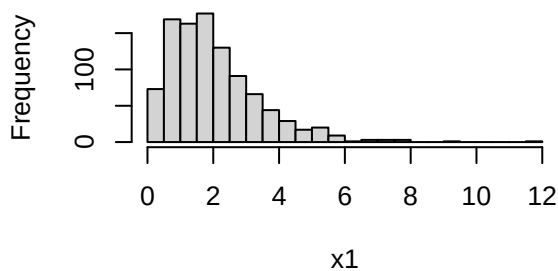
true x_1 marginal
