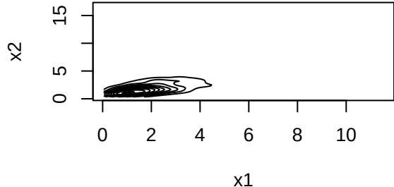
true joint density contour
