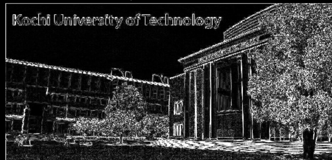
Laplacian Threshold
