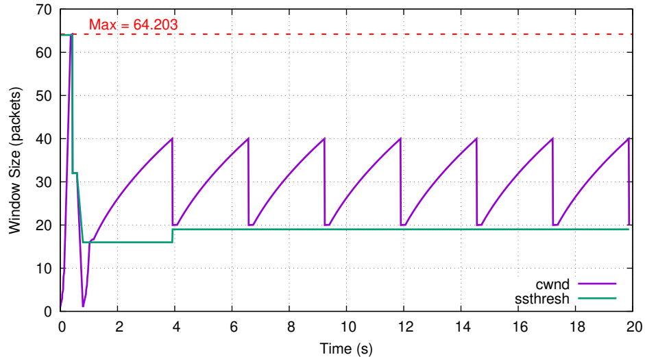
TCP Reno: cwnd and ssthresh
