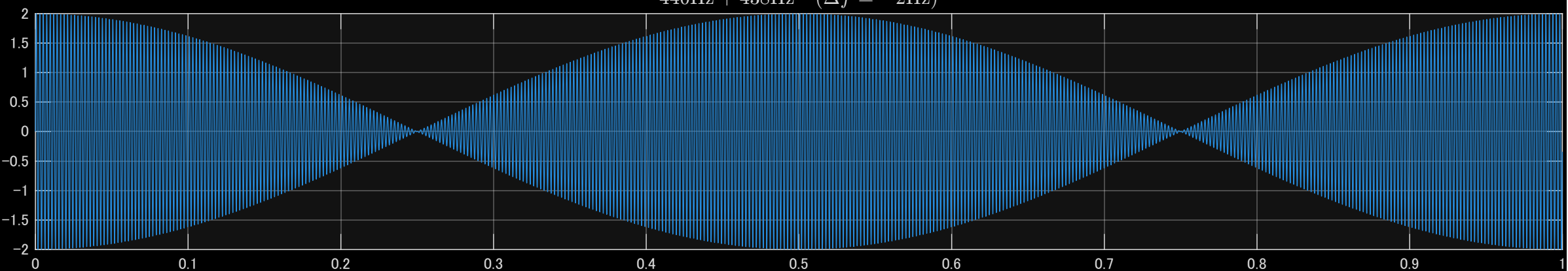
440Hz + 438Hz ( \Delta f = -2\text{Hz} )
