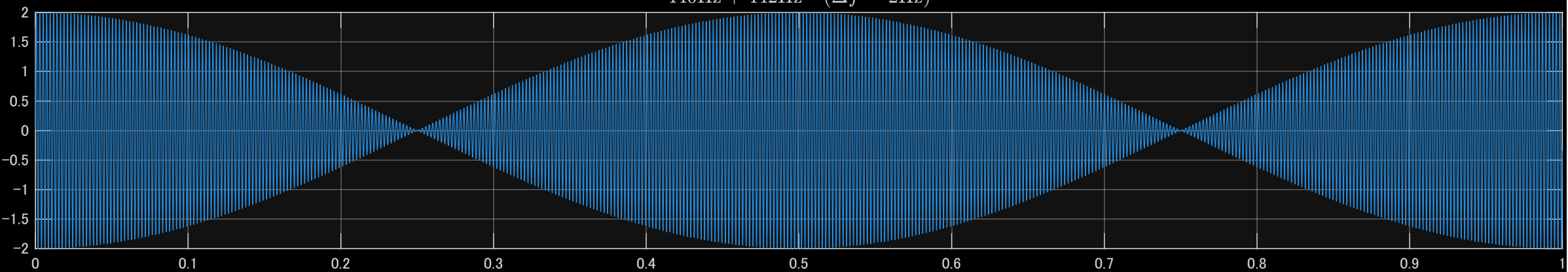
440Hz + 442Hz ( \Delta f = 2\text{Hz} )
