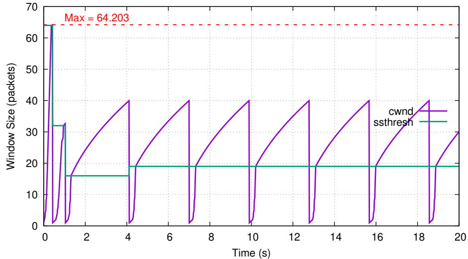
TCP Tahoe: cwnd and ssthresh
